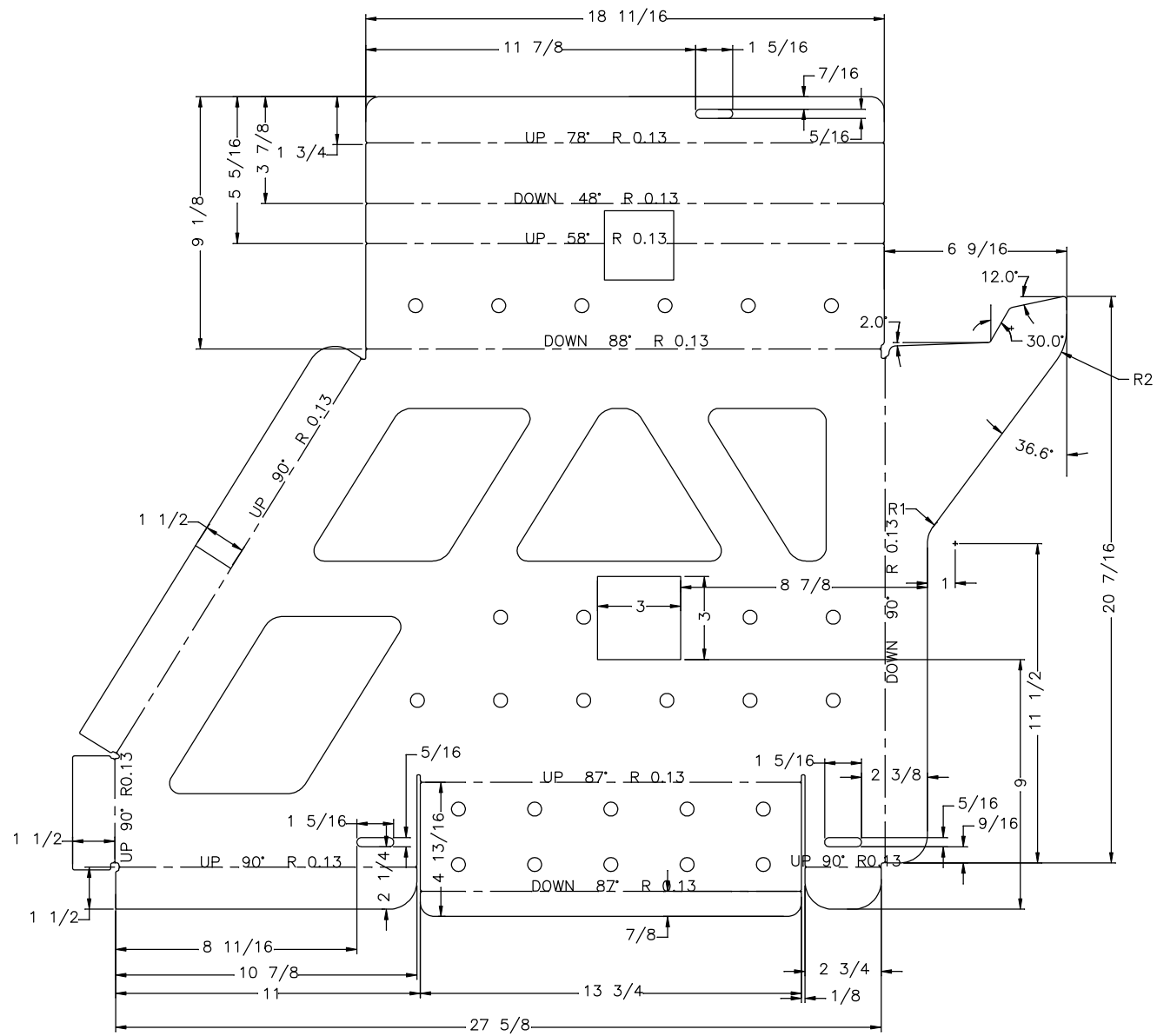
FLAT PATTERN
