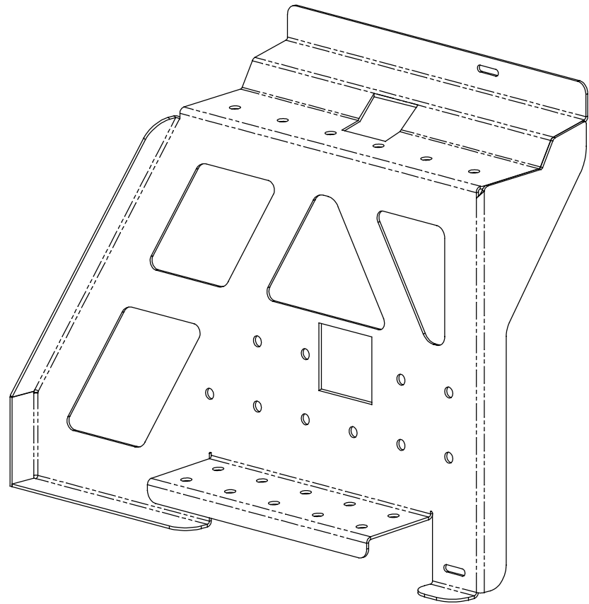
ISO VIEW
