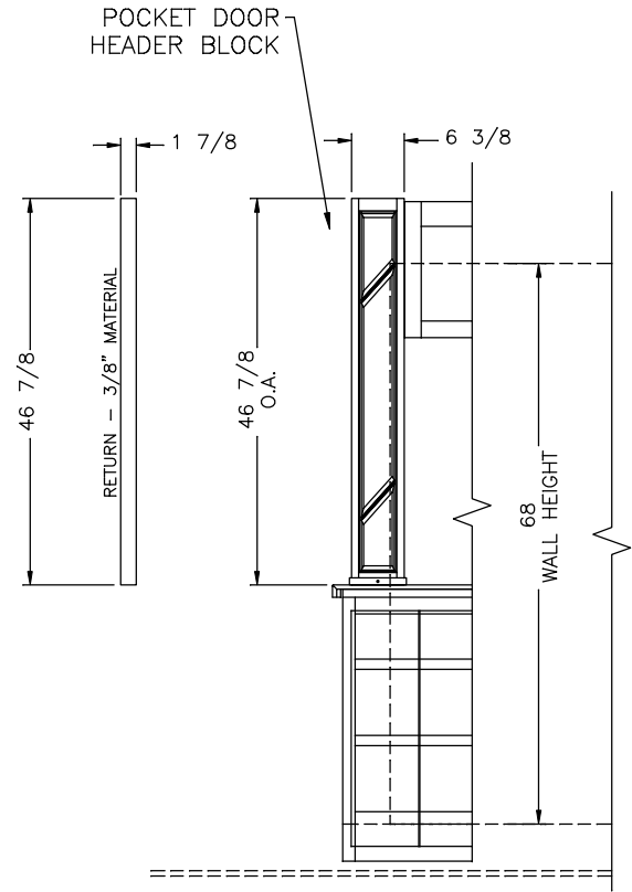
KITCHEN S-O FASCIA (J365)
