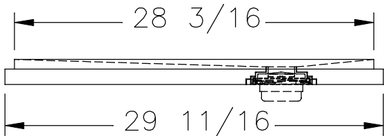
SIDE
