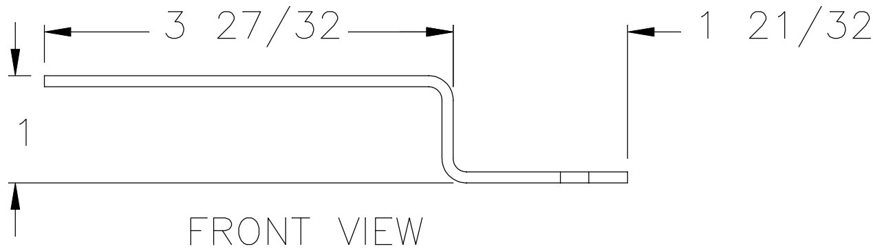
LEFT BRACKET
