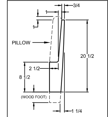
*FRONT OF RAF ARM FRAME DETAIL
