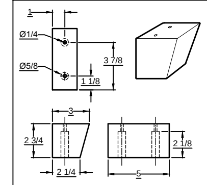
*WOODEN FOOT DETAIL (RAF SIDE) (2:1 SCALE)
