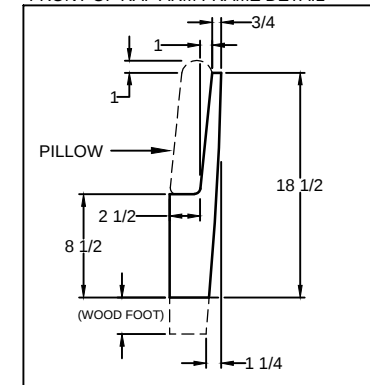
*FRONT OF RAF ARM FRAME DETAIL
