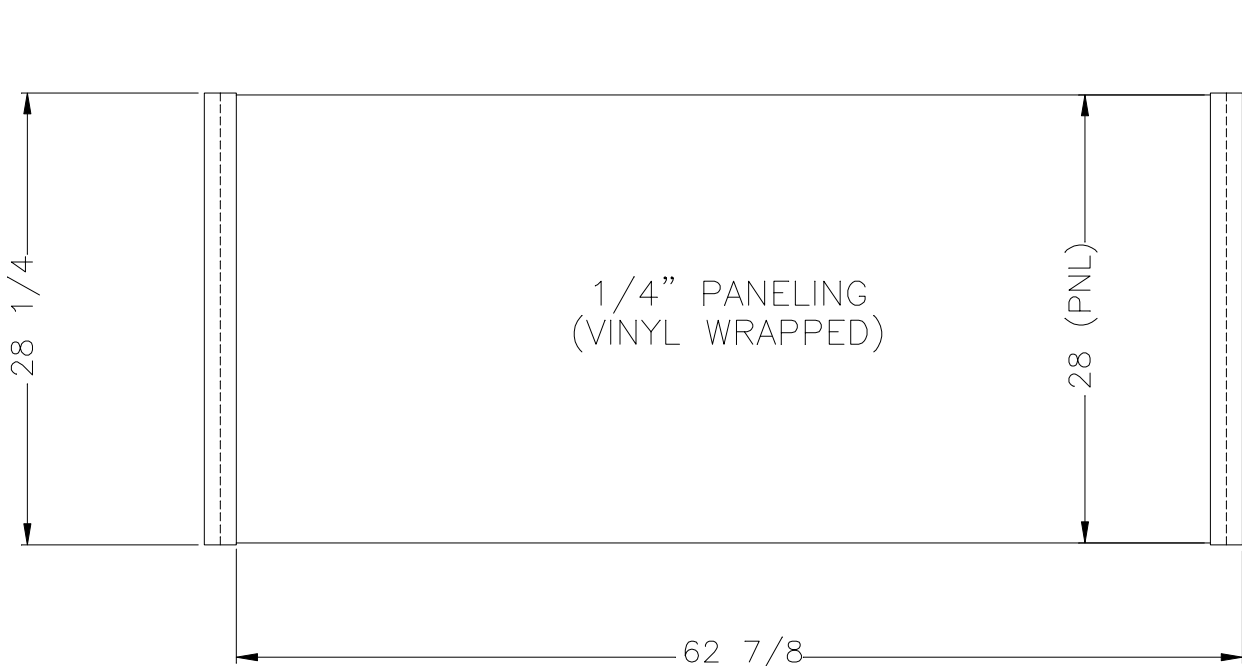
FRONT VIEW
