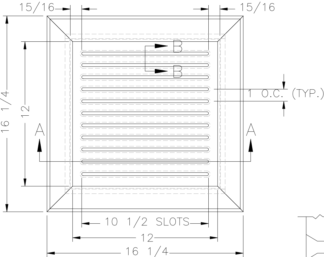
ISO VIEW
