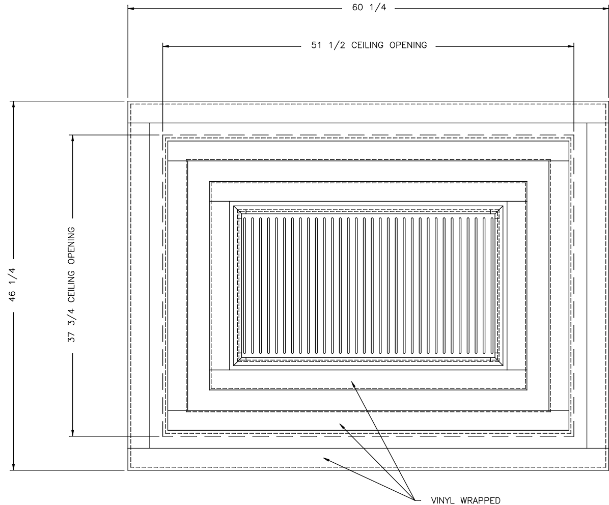
VIEW LOOKING UP AT CEILING
