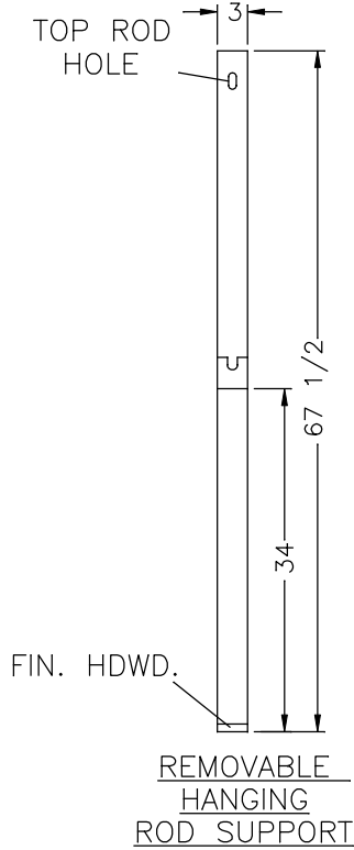
PLAN/FRONT VIEWS
