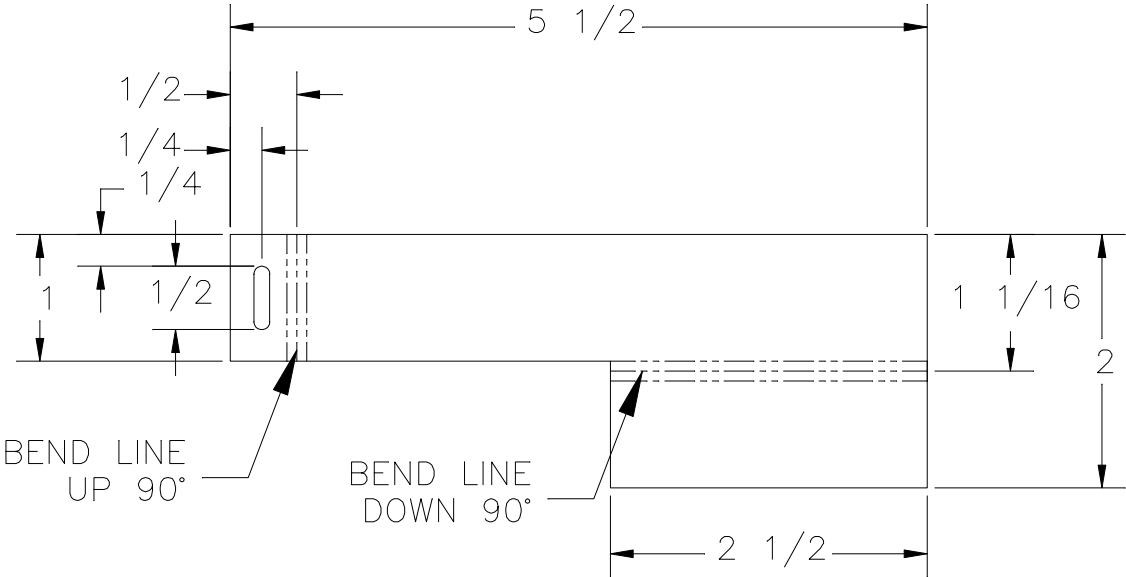
FLAT PATTERN
