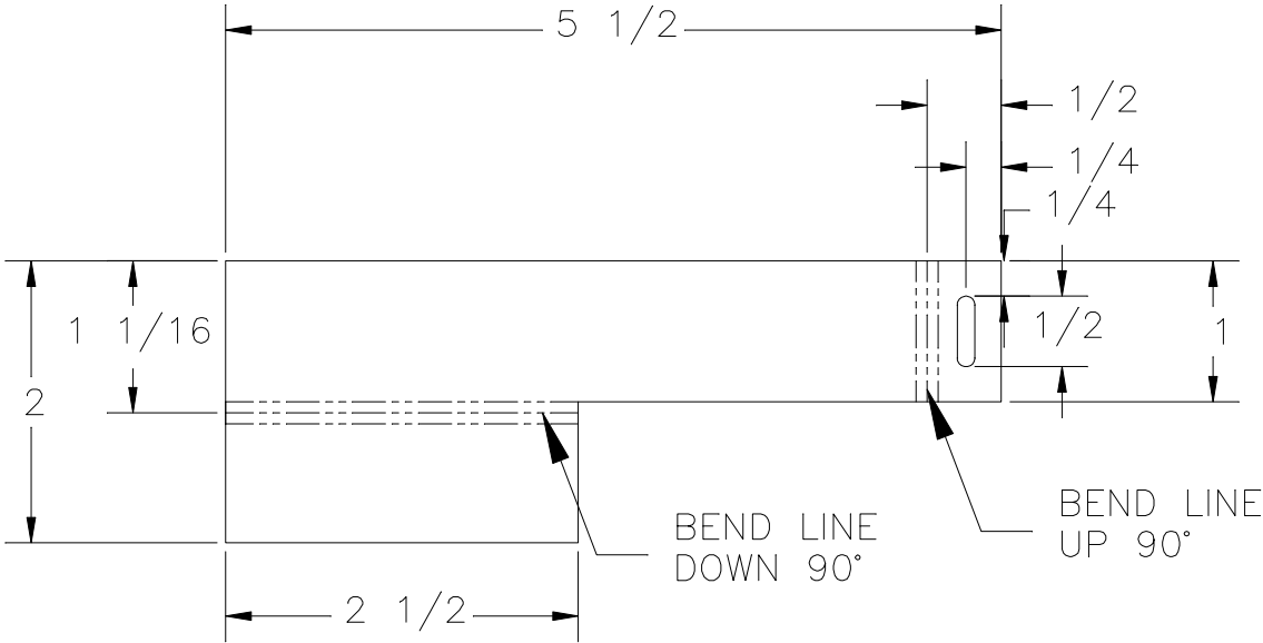
FLAT PATTERN
