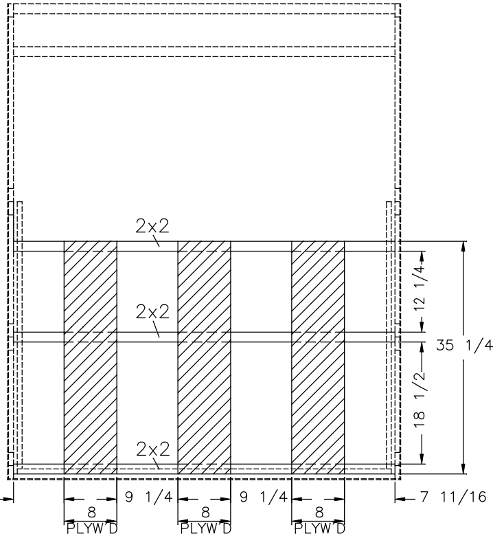
ROLLER BACKER 3/4 PLYWOOD (BOTTOM VIEW)
