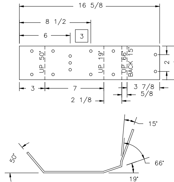
SIDE VIEW BENT PART C (2) REQ'D
