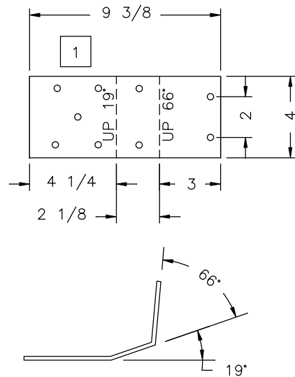
SIDE VIEW BENT PART A (4) REQ'D
