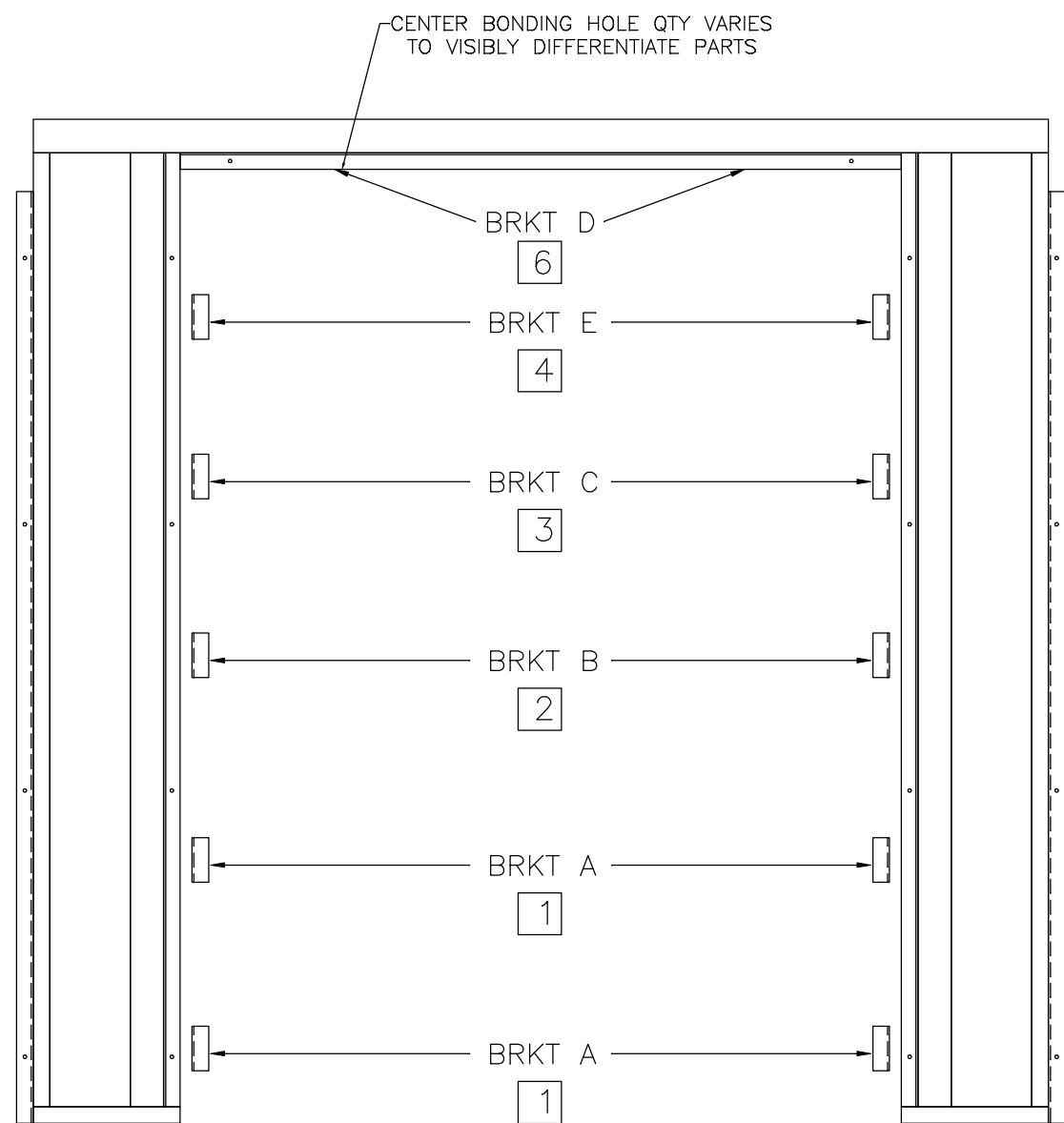
LOCATION OF COLUMN BRACKETS (FRONT WALL NOT DRAWN TO SCALE)
