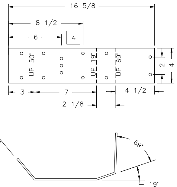
SIDE VIEW BENT PART E (2) REQ'D
