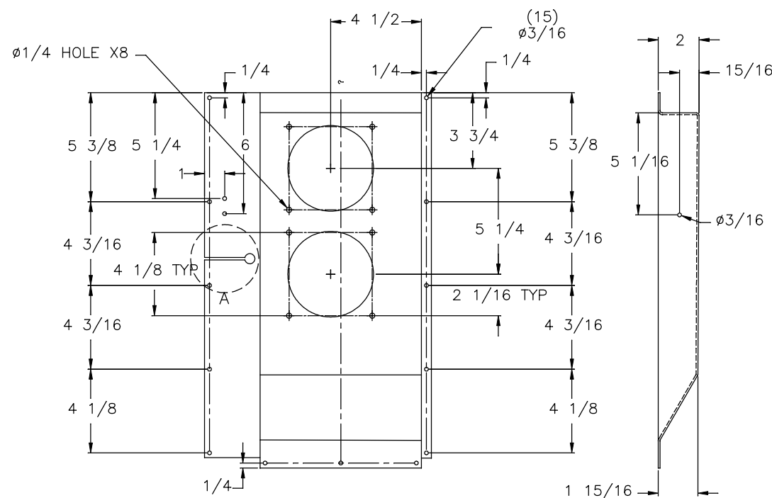
HOLE LOCATIONS
