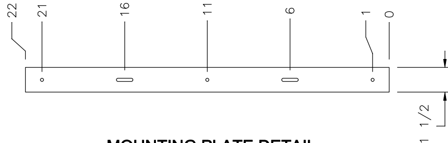
MOUNTING PLATE DETAIL SCALE 2x
