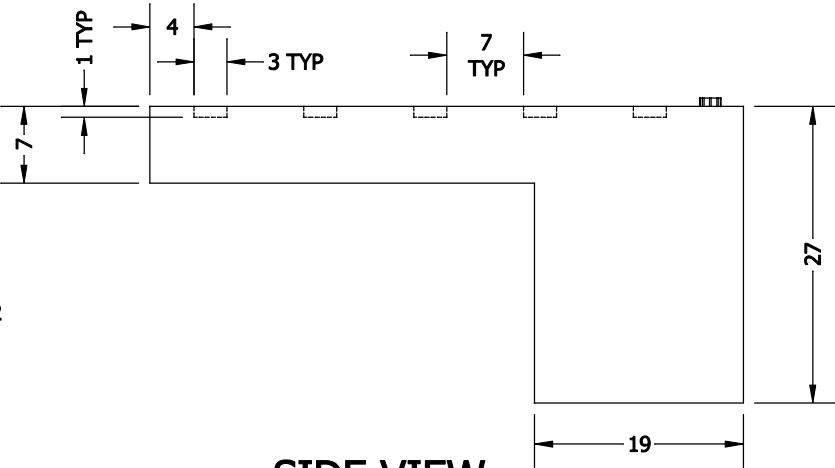
SIDE VIEW
