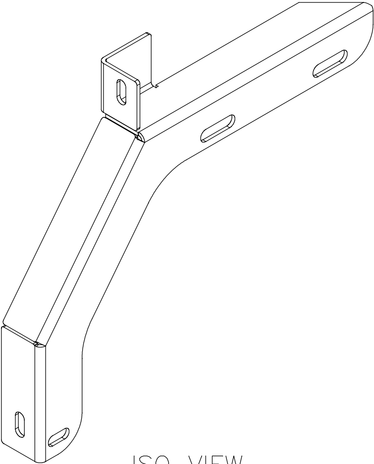
ISO VIEW
