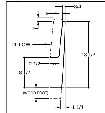
*FRONT OF RAF ARM FRAME DETAIL
