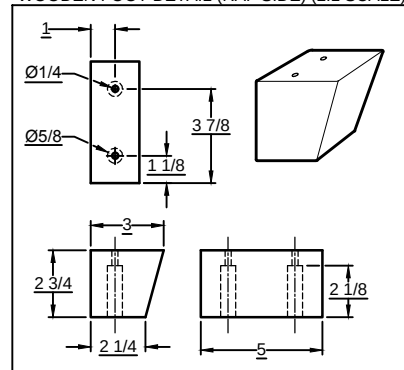
*WOODEN FOOT DETAIL (RAF SIDE) (2:1 SCALE)
