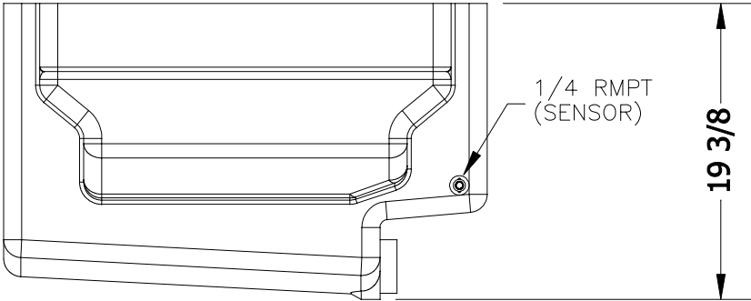
SIDE VIEW
