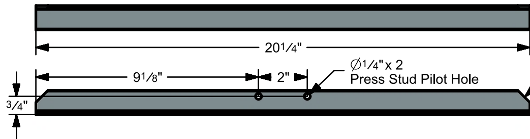
Dual Battery Base Frame Side Angle Matl: 1 x 1 x 1/8 Angle
