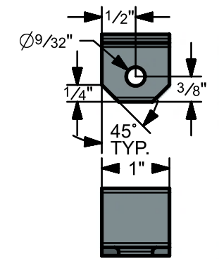
Battery Frame Mounting Tab Matl: 1 x 1 x 1/8 Angle Qty: 4
