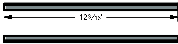
Dual Battery Lower Base Frame Front & Rear Angle Matl: 1/2 x 1/2 x 1/8 Angle Qty: 4
