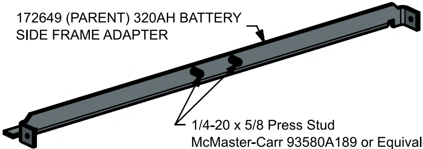
172649 320AH BATTERY SIDE FRAME ADAPTER SUB-ASSEMBLY
