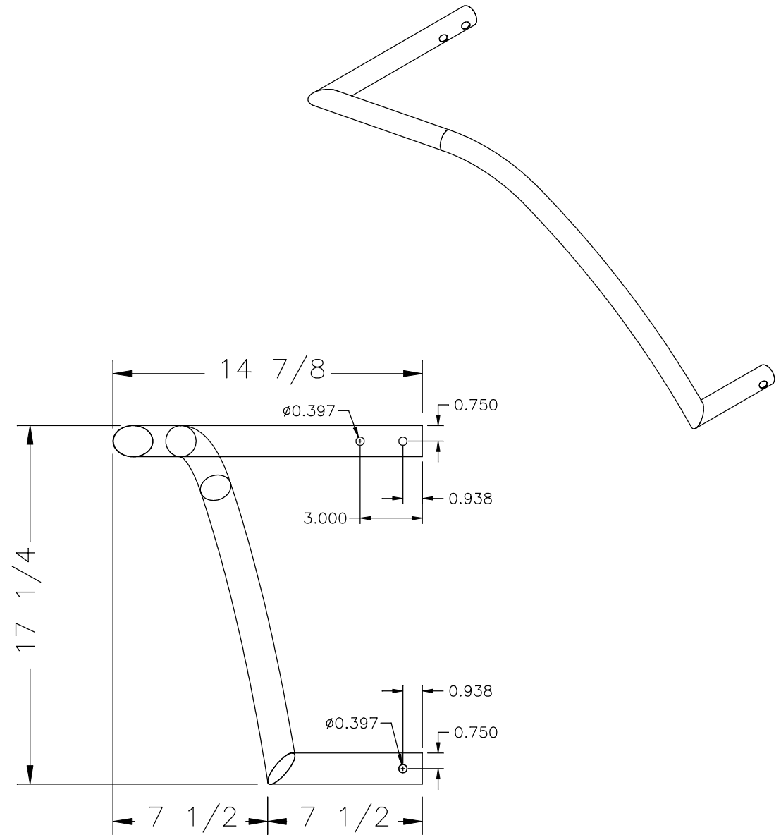
SIDE VIEW
