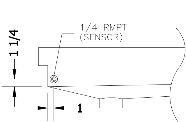
SENSOR LOCATION - VIEW A
