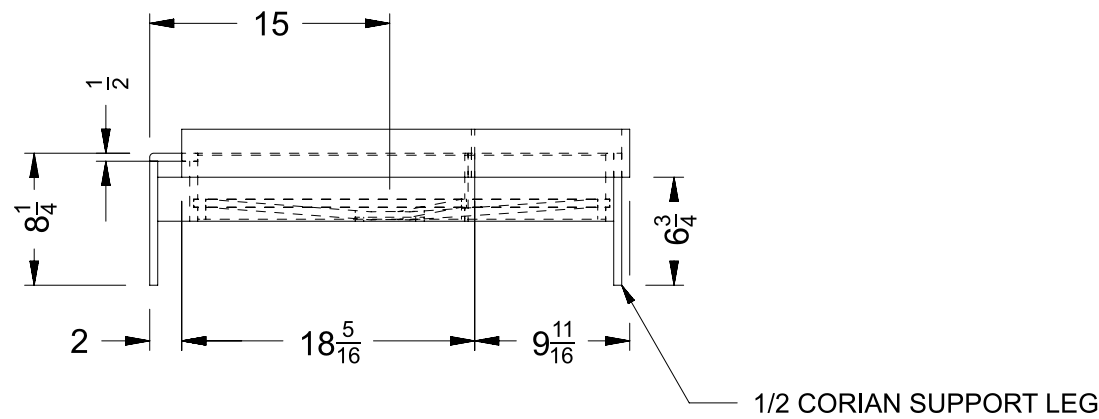
VIEW D
