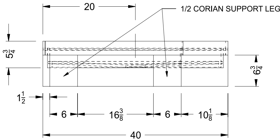
VIEW C
