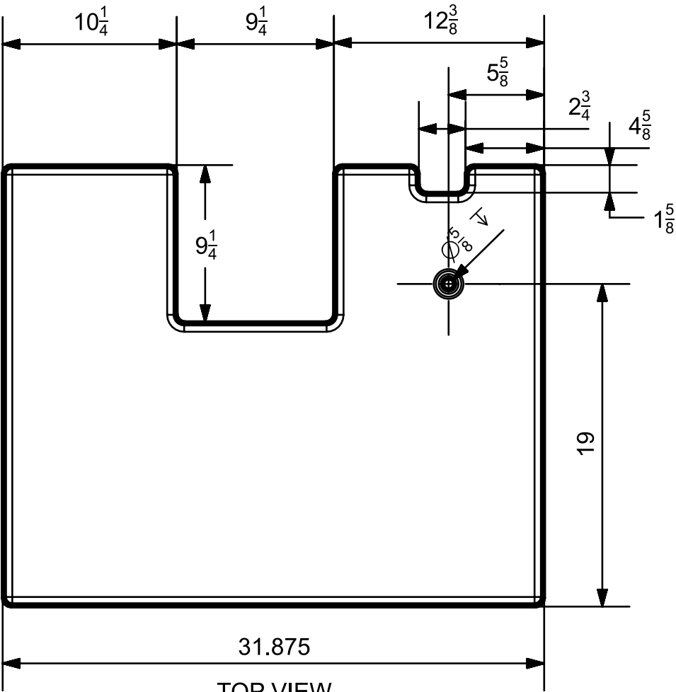
TOP VIEW
