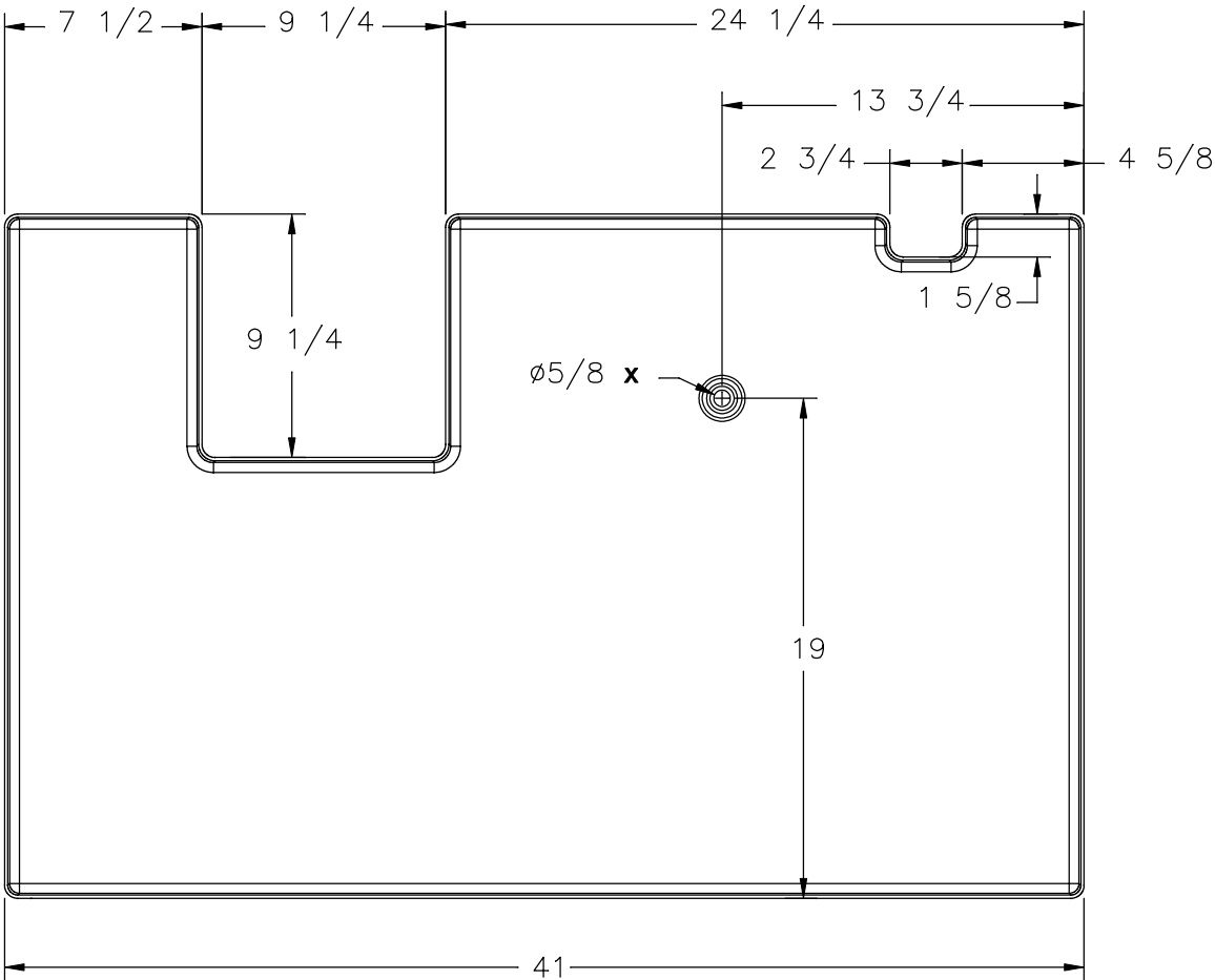
TOP VIEW
