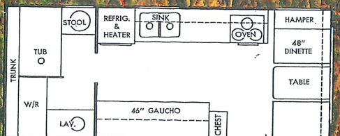
21' REAR BATH TANDEM
