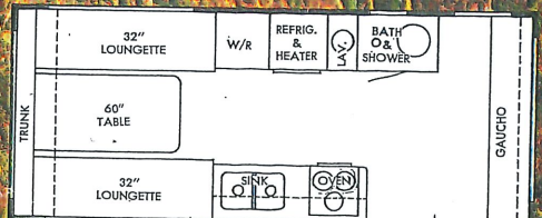
21' TWIN LOUNGE TANDEM
