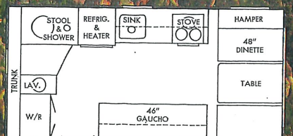
19' REAR BATH
