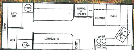
22' F.K. REAR BATH
