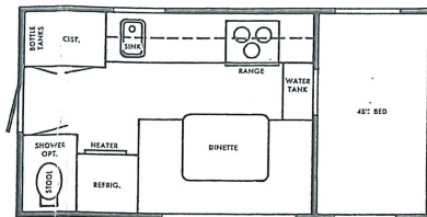
10'6" MODEL
