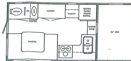
11' MODEL
