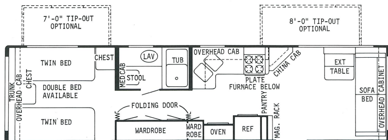
35 CBPK PLAN #1
