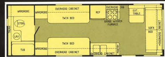
27' REAR BATH
