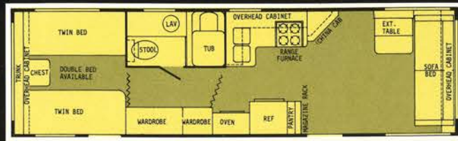
31' CENTER BATH
