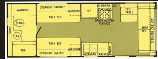
25' REAR BATH
