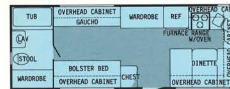
24 Ft. FRONT KITCHEN
