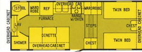
22 Ft. REAR VANITY
