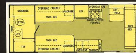
25' REAR BATH
