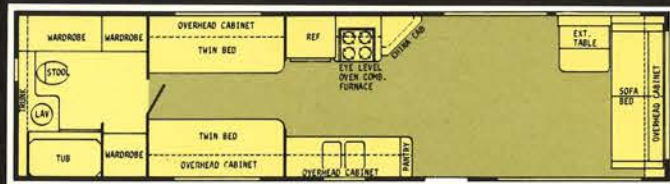
35' REAR BATH
