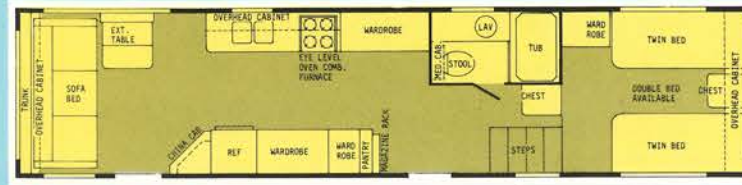
35' FRONT BATH
