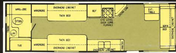
31' REAR BATH
