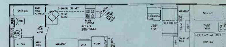
40' REAR BATH FW - PLAN 1
