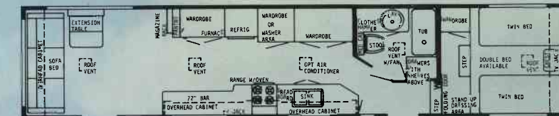
40' FRONT BATH - DOORSIDE KITCHEN FW
