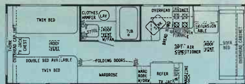
27' CENTER BATH TT
