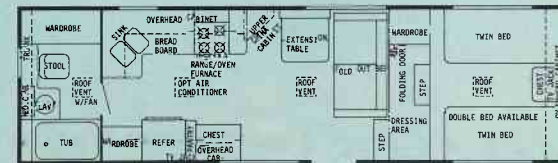
28' REAR BATH FW
