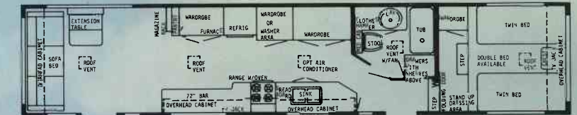
40' FRONT BATH - DOORSIDE KITCHEN FW
