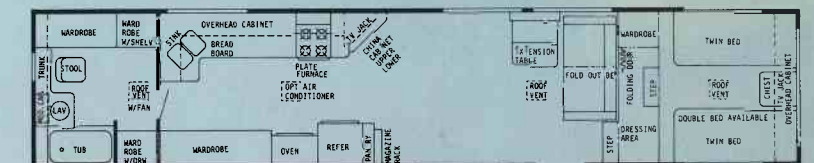
40' REAR BATH FW - PLAN 1
