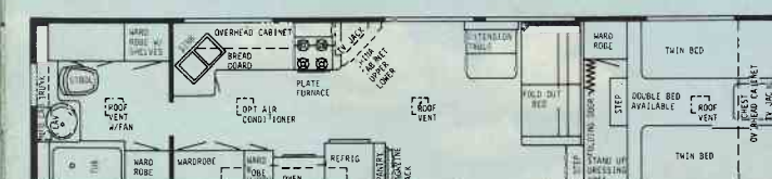
35' REAR BATH FW - PLAN 1
