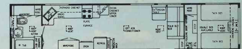
40' REAR BATH FW - PLAN 3
