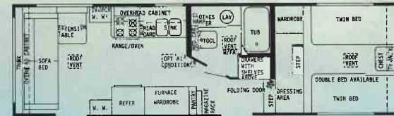
28' FRONT BATH FW
