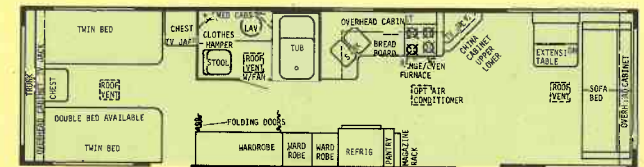
35' CENTER BATH TT
