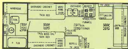
25' REAR BATH TT
