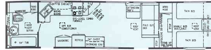
35' REAR BATH – FW – PLAN 3
