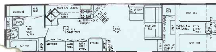
35' REAR BATH – FW – PLAN 1
