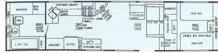
35' REAR BATH – FW – PLAN 2
