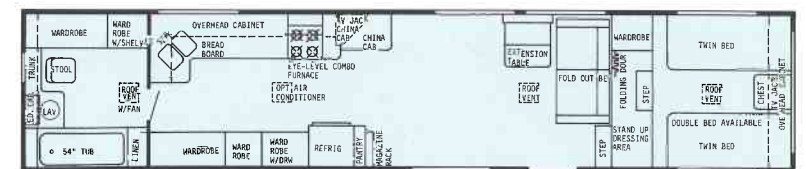
40' REAR BATH – FW – PLAN 1
