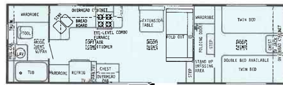
28' REAR BATH – FW
