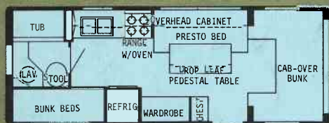
23' Rear Bath Bunk
