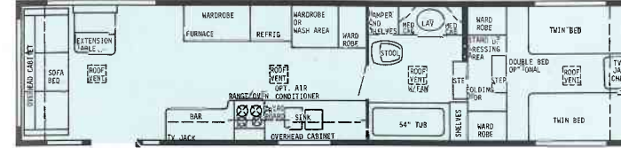
35' WALK-THRU FRONT BATH – FW
