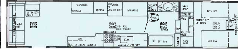
40' WALK-THRU FRONT BATH – FW
