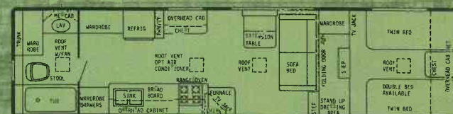
32' REAR BATH DOORSIDE KITCHEN - DRY WT. 7800 lbs. - HITCH WT. 1850 lbs. - OVERALL LENGTH 32' 3"
