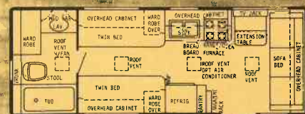
25' REAR BATH T.T. - DRY WT. 5600 lbs. - HITCH WT. 600 lbs. - OVERALL LENGTH 25' 5-1/2"
