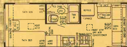
25' CENTER BATH T.T. - DRY WT. 5600 lbs. - HITCH WT. 600 lbs. - OVERALL LENGTH 25' 5-1/2"
