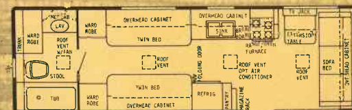
29' REAR BATH T.T. - DRY WT. 6500 lbs. - HITCH WT. 850 lbs. - OVERALL LENGTH 29' 5-1/2"
