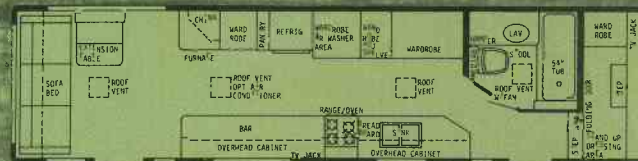
40' FRONT BATH DOORSIDE KITCHEN - DRY WT. 9200 lbs. - HITCH WT. 2000 lbs. - OVERALL LENGTH 39' 7"
