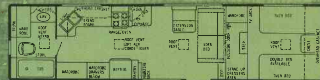
32' REAR BATH - DRY WT. 7800 lbs. - HITCH WT. 1850 lbs. - OVERALL LENGTH 32' 3"
