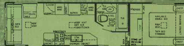
32' FRONT BATH DOORSIDE KITCHEN - DRY WT. 7800 lbs. - HITCH WT. 2000 lbs. - OVERALL LENGTH 32' 3"
