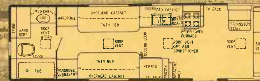
31' REAR BATH T.T. - DRY WT. 6700 lbs. - HITCH WT. 900 lbs. - OVERALL LENGTH 31' 5-1/2"
