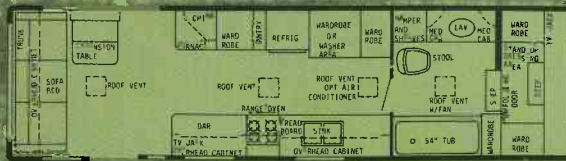
35' WALK THRU FRONT BATH - DRY WT. 8200 lbs. - HITCH WT. 2000 lbs. - OVERALL LENGTH 35' 4"
