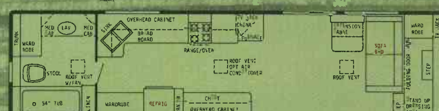
40' REAR BATH PLAN #2 - DRY WT. 9200 lbs. - HITCH WT. 1700 lbs. - OVERALL LENGTH 39' 7"
