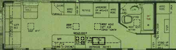
40' FRONT BATH DOORSIDE KITCHEN - DRY WT. 8200 lbs. - HITCH WT. 2000 lbs. - OVERALL LENGTH 39' 7"
