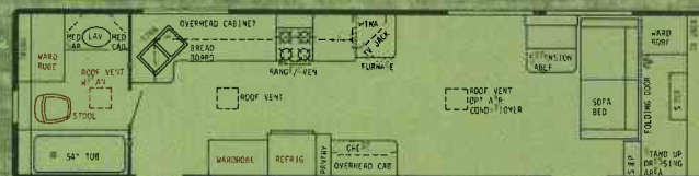
40' REAR BATH PLAN #3 - DRY WT. 9200 lbs. - HITCH WT. 1700 lbs. - OVERALL LENGTH 39' 7"
