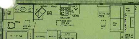
35' REAR BATH PLAN #2 - DRY WT. 8200 lbs. - HITCH WT. 1650 lbs. - OVERALL LENGTH 35' 4"
