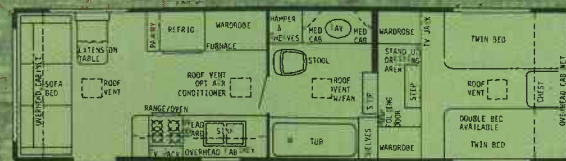
28' WALK THRU FRONT BATH - DRY WT. 7000 lbs. - HITCH WT. 1800 lbs. - OVERALL LENGTH 28' 7-1/2"
