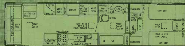
32' WALK THRU FRONT BATH - DRY WT. 7880 lbs. - HITCH WT. 2000 lbs. - OVERALL LENGTH 32' 3"
