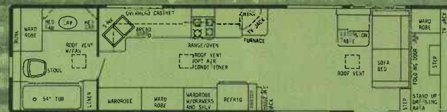
40' REAR BATH PLAN #1 - DRY WT. 9200 lbs. - HITCH WT. 1700 lbs. - OVERALL LENGTH 39' 7"
