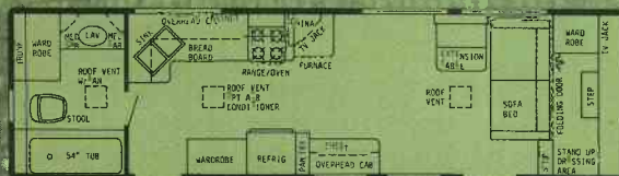
35' REAR BATH PLAN #3 - DRY WT. 8200 lbs. - HITCH WT. 1650 lbs. - OVERALL LENGTH 35' 4"
