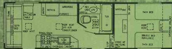
28' FRONT BATH DOORSIDE KITCHEN - DRY WT. 7000 lbs. - HITCH WT. 1800 lbs. - OVERALL LENGTH 28' 7-1/2"
