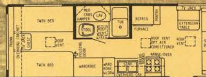
27' CENTER BATH T.T. - DRY WT. 5800 lbs. - HITCH WT. 650 lbs. - OVERALL LENGTH 27' 5-1/2"
