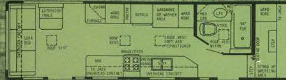
40' FRONT BATH DOORSIDE KITCHEN - DRY WT. 9200 lbs. - HITCH WT. 2000 lbs. - OVERALL LENGTH 39' 7"
