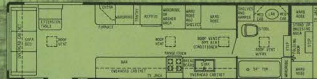
40' WALK THRU FRONT BATH - DRY WT. 9200 lbs. - HITCH WT. 2000 lbs. - OVERALL LENGTH 39' 7"
