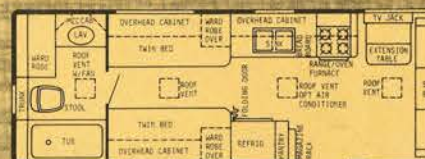
27' REAR BATH T.T. - DRY WT. 5800 lbs. - HITCH WT. 650 lbs. - OVERALL LENGTH 27' 5-1/2"
