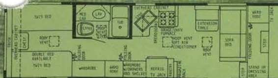
40' CENTER BATH - DRY WT. 9200 lbs. - HITCH WT. 1700 lbs. - OVERALL LENGTH 39' 7"
