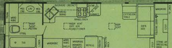
35' REAR BATH PLAN #1 - DRY WT. 8200 lbs. - HITCH WT. 1650 lbs. - OVERALL LENGTH 35' 4"
