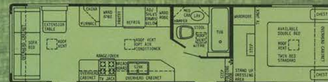
32' FRONT BATH DOORSIDE KITCHEN - DRY WT. 7800 lbs. - HITCH WT. 2000 lbs. - OVERALL LENGTH 32' 3"
