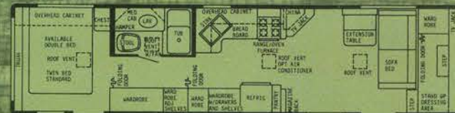
40' CENTER BATH - DRY WT. 9200 lbs. - HITCH WT. 1700 lbs. - OVERALL LENGTH 39' 7"
