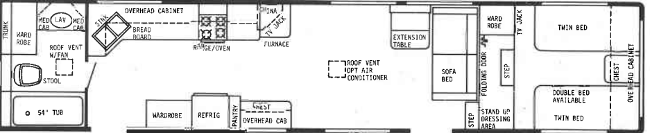
40' REAR BATH PLAN #3-GVWR 13,000 lbs.-HITCH WT. 1700 lbs.-OVERALL LENGTH 39' 7"
