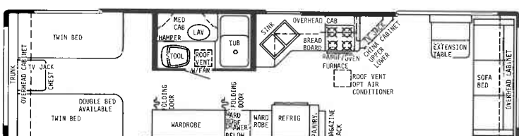
35' CENTER BATH T.T.-GVWR 9000 lbs.-HITCH WT. 850 lbs.-OVERALL LENGTH 34' 6-1/2"
