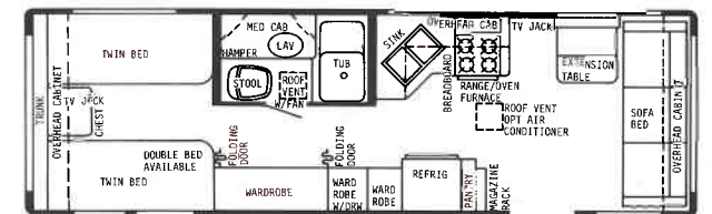
29' CENTER BATH T.T.-GVWR 9000 lbs. HITCH WT. 850 lbs. OVERALL LENGTH 29' 5-1/2"
