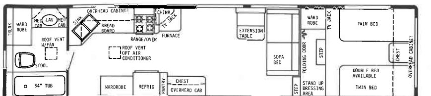
35' REAR BATH PLAN #3-GVWR 11,000 lbs.-HITCH WT. 1650 lbs.-OVERALL LENGTH 35' 4"
