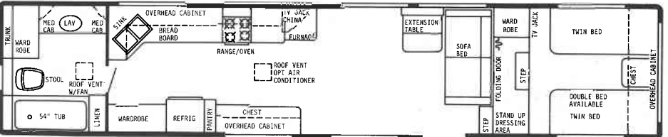
40' REAR BATH PLAN #2-GVWR 13,000 lbs.-HITCH WT. 1700 lbs.-OVERALL LENGTH 39' 7"
