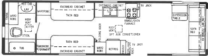
33' REAR BATH-GVWR 9000 lbs.-HITCH WT. 900 lbs.-OVERALL LENGTH 33' 5"
