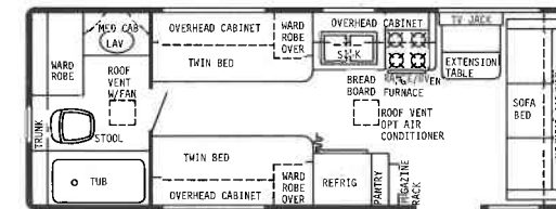
25' REAR BATH T.T.-GVWR 8000 lbs. HITCH WT. 600 lbs. OVERALL LENGTH 25' 5-1/2"
