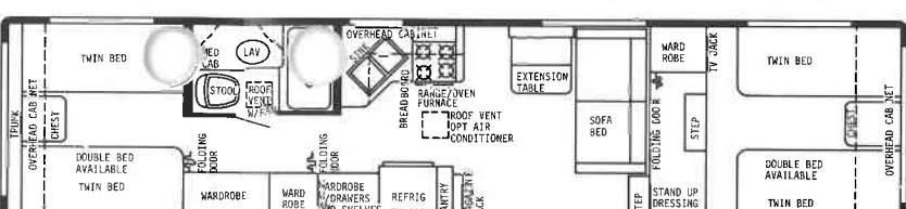
35' CENTER BATH-GVWR 11,000 lbs.-HITCH WT. 1650 lbs.-OVERALL LENGTH 35' 4"
