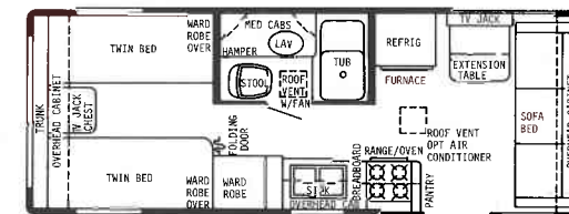
25' CENTER BATH T.T.-GVWR 8000 lbs. HITCH WT. 600 lbs. OVERALL LENGTH 25' 5-1/2"
