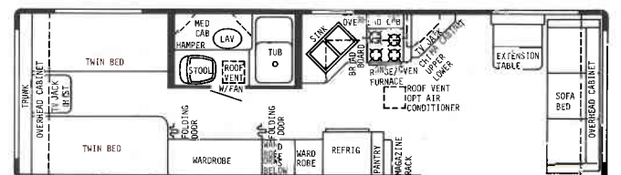
31' CENTER BATH T.T.-GVWR 9000 lbs. HITCH WT. 900 lbs. OVERALL LENGTH 31' 5-1/2"
