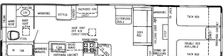
32' REAR BATH DOORSIDE KITCHEN-GVWR 10,000 lbs.-HITCH WT. 1850 lbs.-OVERALL LENGTH 32' 3"
