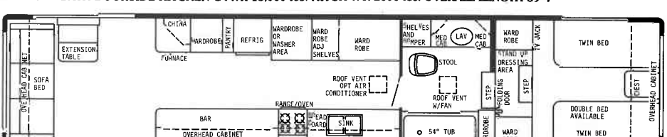
40' WALK THRU FRONT BATH-GVWR 13,000 lbs.-HITCH WT. 2000 lbs.-OVERALL LENGTH 39' 7"
