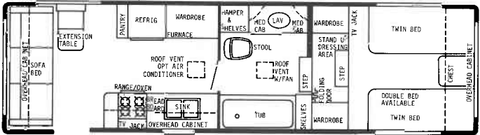
28' WALK THRU FRONT BATH-GVWR 10,000 lbs.-HITCH WT. 1800 lbs.-OVERALL LENGTH 28' 7-1/2"
