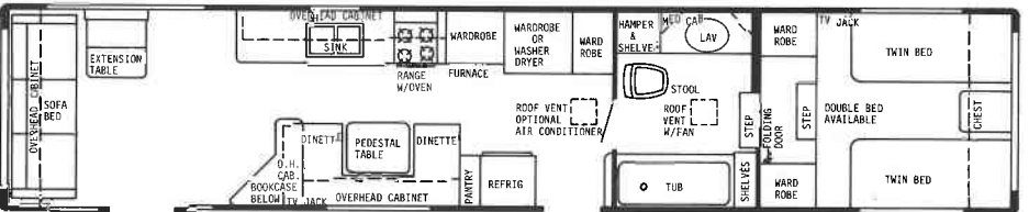
40' WALK THRU FRONT BATH-2 DOOR-GVWR 13,000 lbs.-HITCH WT. 2000 lbs.-OVERALL LENGTH 39' 7"
