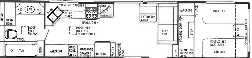
35' REAR BATH PLAN #1-GVWR 11,000 lbs.-HITCH WT. 1650 lbs.-OVERALL LENGTH 35' 4"
