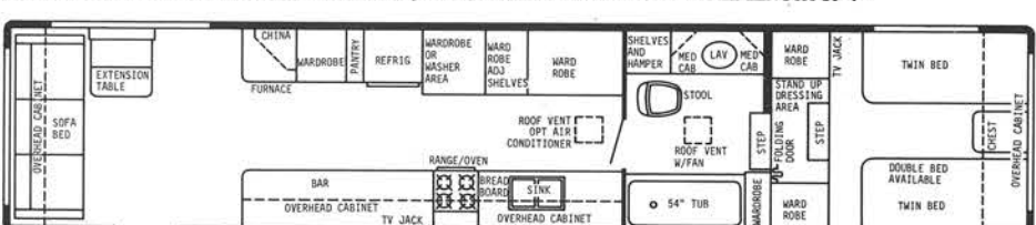
40' WALK THRU FRONT BATH-2 DOOR-GVWR 13,000 lbs.-HITCH WT. 2000 lbs.-OVERALL LENGTH 39' 7"
