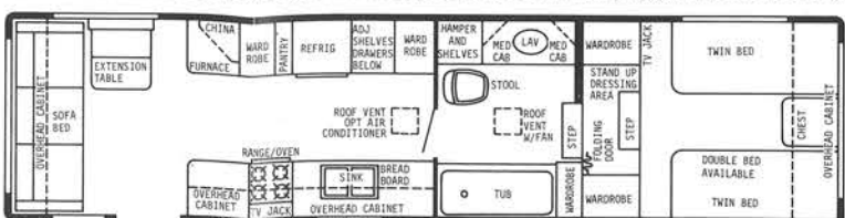
32' WALK THRU FRONT BATH-GVWR 10,000 lbs.-HITCH WT. 2000 lbs.-OVERALL LENGTH 32' 3"
