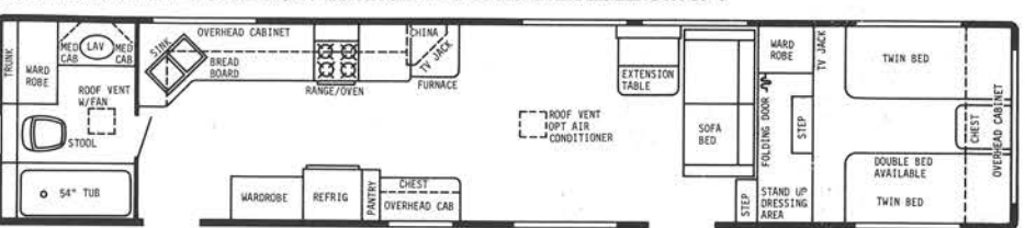
40' REAR BATH PLAN #3-GVWR 13,000 lbs.-HITCH WT. 1700 lbs.-OVERALL LENGTH 39' 7"
