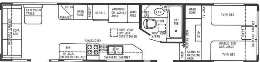
35' FRONT BATH DOORSIDE KITCHEN-GVWR 11,000 lbs.-HITCH WT. 2000 lbs.-OVERALL LENGTH 35' 4"
