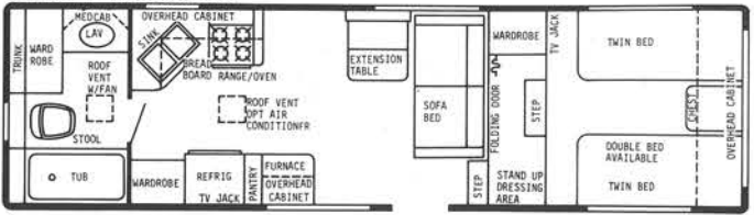
28' REAR BATH-GVWR 10,000 lbs.-HITCH WT. 1800 lbs.-OVERALL LENGTH 28' 7-1/2"
