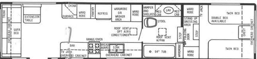
35' WALK THRU FRONT BATH-GVWR 11,000 lbs.-HITCH WT. 2000 lbs.-OVERALL LENGTH 35' 4"
