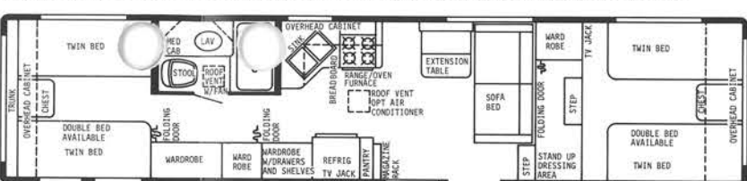
35' CENTER BATH-GVWR 11,000 lbs.-HITCH WT. 1650 lbs.-OVERALL LENGTH 35' 4"
