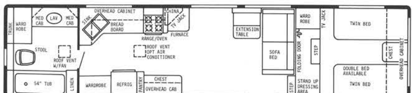
35' REAR BATH PLAN #2-GVWR 11,000 lbs.-HITCH WT. 1650 lbs.-OVERALL LENGTH 35' 4"
