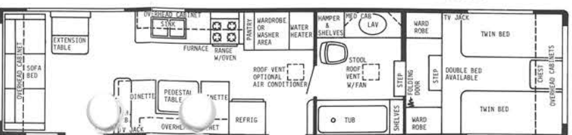
35' WALK THRU FRONT BATH-2DOOR-GVWR 11,000 lbs.-HITCH WT. 2000 lbs.-OVERALL LENGTH 35' 4"
