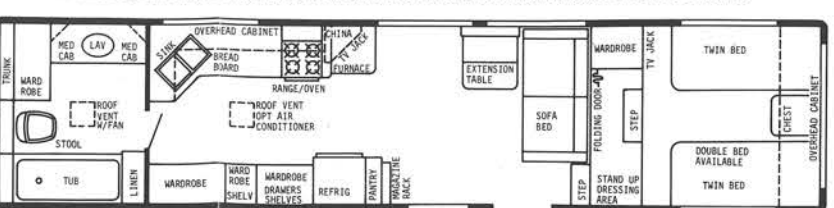
35' REAR BATH PLAN #1-GVWR 11,000 lbs.-HITCH WT. 1650 lbs.-OVERALL LENGTH 35' 4"
