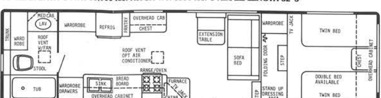
32' REAR BATH DOORSIDE KITCHEN-GVWR 10,000 lbs.-HITCH WT. 1850 lbs.-OVERALL LENGTH 32' 3"
