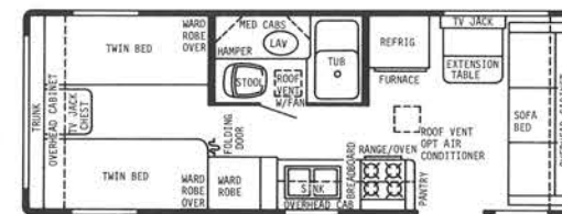
25' CENTER BATH T.T. GVWR 8000 lbs. HITCH WT. 600 lbs. OVERALL LENGTH 25' 5-1/2"
