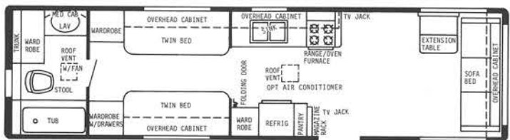
33' REAR BATH-GVWR 9000 lbs.-HITCH WT. 900 lbs.-OVERALL LENGTH 33' 5"
