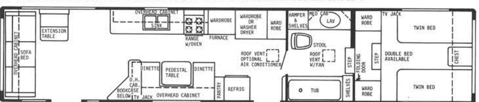
40' REAR BATH PLAN #1-GVWR 13,000 lbs.-HITCH WT. 1700 lbs.-OVERALL LENGTH 39' 7"
