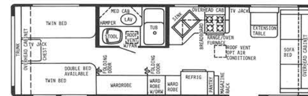
29' CENTER BATH T.T. GVWR 9000 lbs. HITCH WT. 850 lbs. OVERALL LENGTH 29' 5-1/2"
