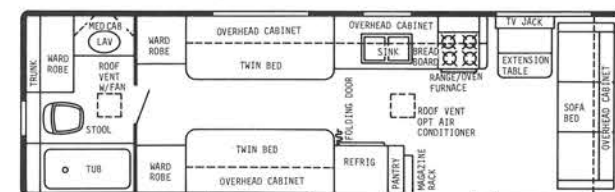
29' REAR BATH T.T. GVWR 9000 lbs. HITCH WT. 850 lbs. OVERALL LENGTH 29' 5-1/2"
