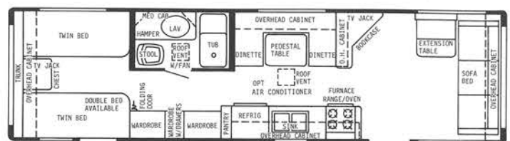
33' CENTER BATH DINETTE-GVWR 9000 lbs.-HITCH WT. 900 lbs.-OVERALL LENGTH 33' 5"
