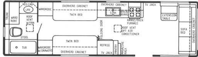
31' REAR BATH T.T.-GVWR 9000 lbs.-HITCH WT. 900 lbs.-OVERALL LENGTH 31' 5-1/2"
