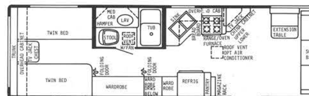
31' CENTER BATH T.T. GVWR 9000 lbs. HITCH WT. 900 lbs. OVERALL LENGTH 31' 5-1/2"
