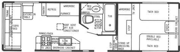
28' FRONT BATH DOORSIDE KITCHEN-GVWR 10,000 lbs. - HITCH WT. 1800 lbs.-OVERALL LENGTH 28' 7-1/2"
