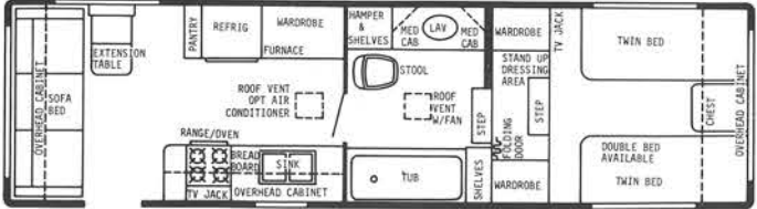
28' WALK THRU FRONT BATH-GVWR 10,000 lbs.-HITCH WT. 1800 lbs.-OVERALL LENGTH 28' 7-1/2"
