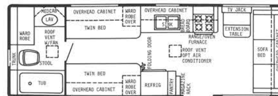
27' REAR BATH T.T. GVWR 8000 lbs. HITCH WT. 650 lbs. OVERALL LENGTH 27' 5-1/2"
