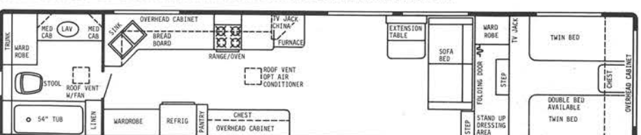
40' REAR BATH PLAN #3-GVWR 13,000 lbs.-HITCH WT. 1700 lbs.-OVERALL LENGTH 39' 7"
