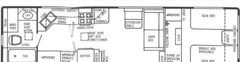
32' REAR BATH-GVWR 10,000 lbs.-HITCH WT. 1850 lbs.-OVERALL LENGTH 32' 3"
