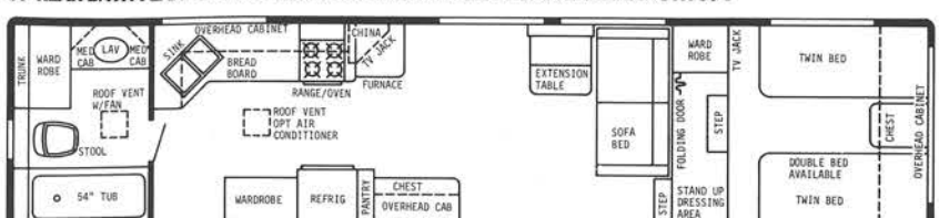
35' REAR BATH PLAN #3-GVWR 11,000 lbs.-HITCH WT. 1650 lbs.-OVERALL LENGTH 35' 4"
