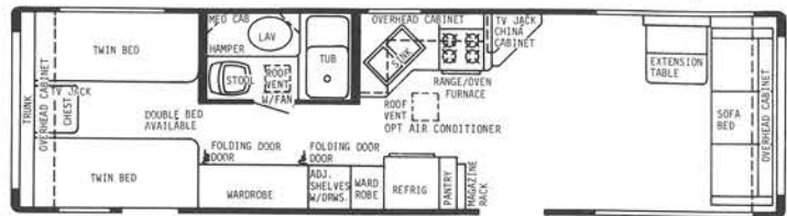
33' CENTER BATH-GVWR 9000 lbs.-HITCH WT. 900 lbs.-OVERALL LENGTH 33' 5"
