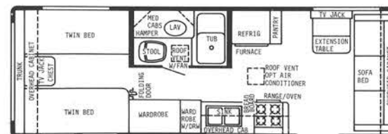
27' CENTER BATH T.T. GVWR 8000 lbs. HITCH WT. 650 lbs. OVERALL LENGTH 27' 5-1/2"
