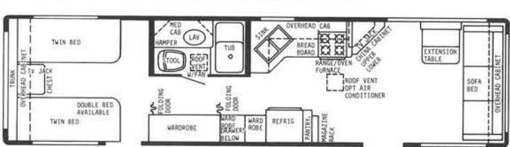
35' CENTER BATH T.T.-GVWR 9000 lbs.-HITCH WT. 850 lbs.-OVERALL LENGTH 34' 6-1/2"
