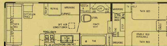
28' WALK-THRU FRONT BATH - GVWR 10,000 lbs. - HITCH WT. 1800 lbs. - OVERALL LENGTH 28'8"
