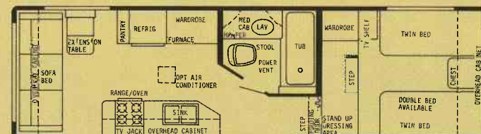
28' FRONT BATH DOORSIDE KITCHEN - GVWR 10,000 lbs. - HITCH WT. 1800 lbs. - OVERALL LENGTH 28'8"
