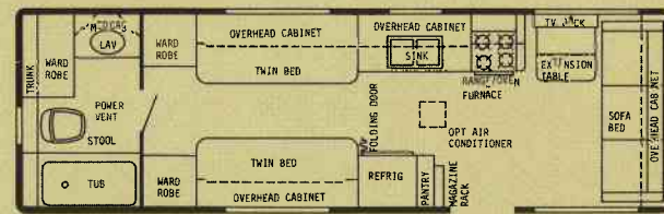
29' REAR BATH - GVWR 9000 lbs. - HITCH WT. 675 lbs. - OVERALL LENGTH 29'5"
