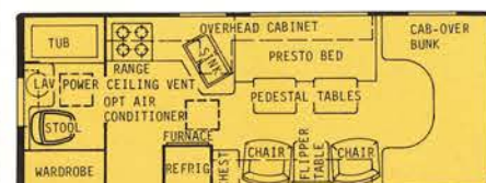
23BRD DRY WT. 9600 lbs. (approx.) OVERALL LENGTH 24'4"
