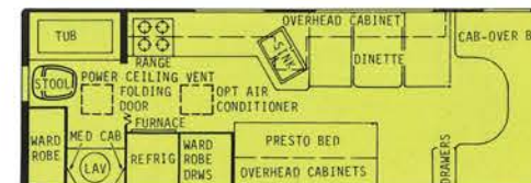
28RB DRY WT. 10,000 lbs. (approx.) OVERALL LENGTH 27'4"
