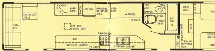
40' FRONT BATH DOORSIDE KITCHEN - GVWR 12,000 lbs. - HITCH WT. 2000 lbs. - OVERALL LENGTH 39'6"
