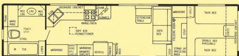
35' REAR BATH PLAN #1 - GVWR 11,000 lbs. - HITCH WT. 1800 lbs. - OVERALL LENGTH 35'6"
