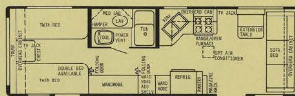
29' CENTER BATH - GVWR 9000 lbs. - HITCH WT. 675 lbs. - OVERALL LENGTH 29'5"
