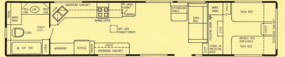
40' REAR BATH PLAN #2 - GVWR 12,000 lbs. - HITCH WT. 1750 lbs. - OVERALL LENGTH 39'6"
