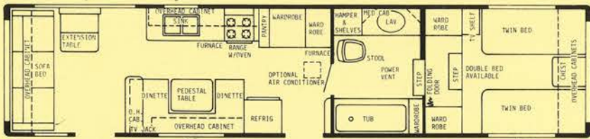
35' WALK-THRU FRONT BATH - 2 DOOR - GVWR 11,000 lbs. - HITCH WT. 2000 lbs. - OVERALL LENGTH 35'6"
