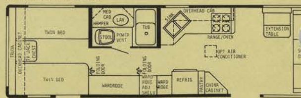
31' CENTER BATH - GVWR 9000 lbs. - HITCH WT. 700 lbs. - OVERALL LENGTH 31'5"
