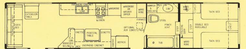
40' WALK-THRU FRONT BATH - 2 DOOR - GVWR 12,000 lbs. - HITCH WT. 2000 lbs. - OVERALL LENGTH 39'6"
