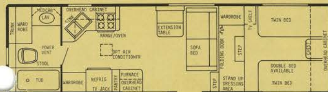
28' REAR BATH - GVWR 10,000 lbs. - HITCH WT. 1800 lbs. - OVERALL LENGTH 28'8"
