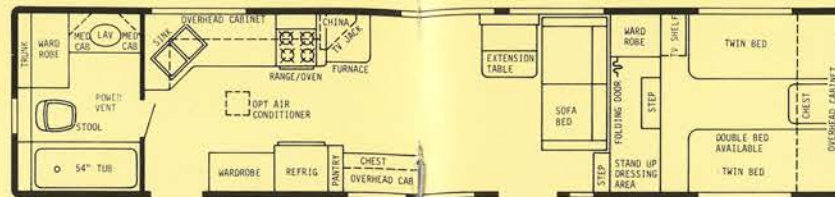
35' REAR BATH PLAN #3 - GVWR 11,000 lbs. - HITCH WT. 1800 lbs. - OVERALL LENGTH 35'6"
