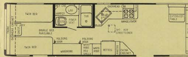
33' CENTER BATH - GVWR 9000 lbs. - HITCH WT. 700 lbs. - OVERALL LENGTH 33'5"
