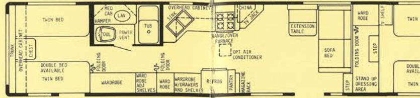
40' CENTER BATH - GVWR 12,000 lbs. - HITCH WT. 1750 lbs. - OVERALL LENGTH 39'6"
