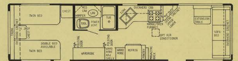
35' CENTER BATH - GVWR 9000 lbs. - HITCH WT. 700 lbs. - OVERALL LENGTH 34'6"
