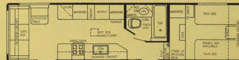
32' FRONT BATH DOORSIDE KITCHEN - GVWR 10,000 lbs. - HITCH WT. 2000 lbs. - OVERALL LENGTH 32'6"
