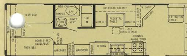
33' CENTER BATH DINETTE - GVWR 9000 lbs. - HITCH WT. 700 lbs. - OVERALL LENGTH 33'5"
