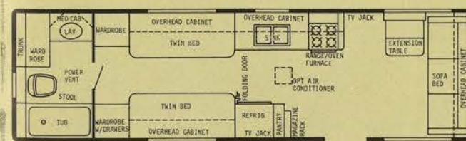
31' REAR BATH - GVWR 9000 lbs. - HITCH WT. 700 lbs. - OVERALL LENGTH 31'5"
