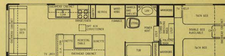
32' WALK-THRU FRONT BATH 2-DOOR - GVWR 10,000 lbs. - HITCH WT. 2000 lbs. - OVERALL LENGTH 32'6"
