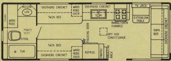
27' REAR BATH - GVWR 8000 lbs. - HITCH WT. 550 lbs. - OVERALL LENGTH 27'5"
