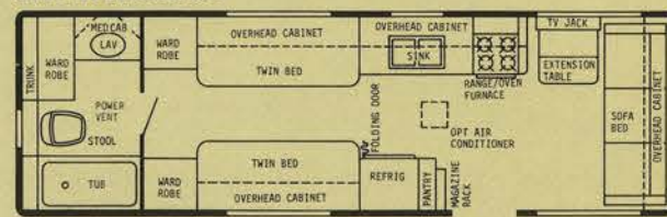
29' REAR BATH - GVWR 9000 lbs. - HITCH WT. 675 lbs. - OVERALL LENGTH 29'5"
