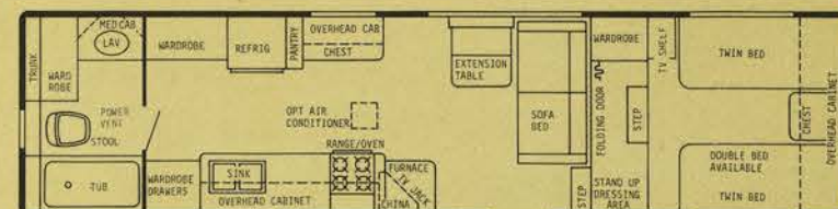
32' REAR BATH DOORSIDE KITCHEN - GVWR 10,000 lbs. - HITCH WT. 1750 lbs. - OVERALL LENGTH 32'6"
