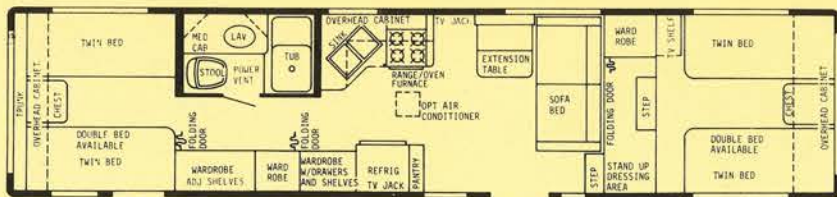
35' CENTER BATH - GVWR 11,000 lbs. - HITCH WT. 1800 lbs. - OVERALL LENGTH 35'6"
