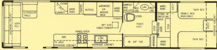
35' WALK-THRU FRONT BATH - GVWR 11,000 lbs. - HITCH WT. 2000 lbs. - OVERALL LENGTH 35'6"
