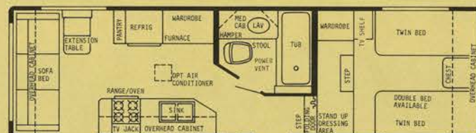
28' FRONT BATH DOORSIDE KITCHEN - GVWR 10,000 lbs. - HITCH WT. 1800 lbs. - OVERALL LENGTH 28'8"
