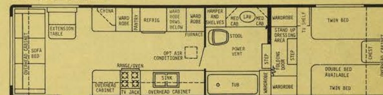
32' WALK-THRU FRONT BATH - GVWR 10,000 lbs. - HITCH WT. 2000 lbs. - OVERALL LENGTH 32'6"
