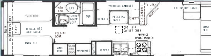
35' Center Bath Dinette - Dry Wt. 7000 lbs. - Hitch Wt. 700 lbs. - Overall Length 34'6"
