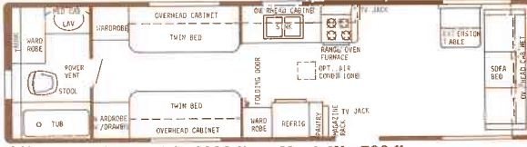
33' Rear Bath - Dry Wt. 6900 lbs. - Hitch Wt. 700 lbs. - Overall Length 33'5"
