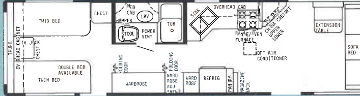
35' Center Bath - Dry Wt. 7000 lbs. - Hitch Wt. 700 lbs. - Overall Length 34'6"
