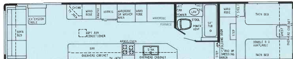
40' Front Bath Doorside Kitchen - Dry Wt. 9300 lbs. - Hitch Wt. 1650 lbs. - Overall Length 39'6"
