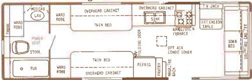
29' Rear Bath - Dry Wt. 6500 lbs. - Hitch Wt. 675 lbs. - Overall Length 29'5"
