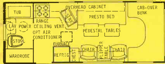
23RBRD - Dry Wt. 9600 lbs. - Overall length 24'4"
