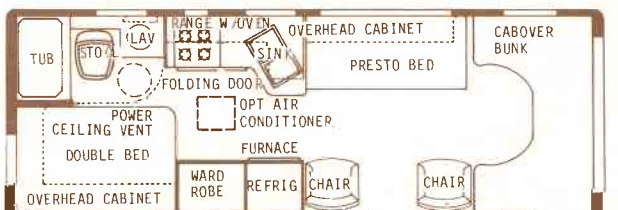
26RBDDB - Dry Wt. 9800 lbs. - Overall length 26'4"
