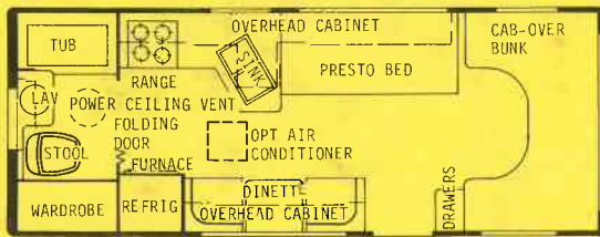
23RB - Dry Wt. 9600 lbs. - Overall length 24'4"
