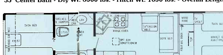
35' Walk-Thru Center Bath - Dry Wt. 8500 lbs. - Hitch Wt. 1650 lbs. - Overall Length 35'6"
