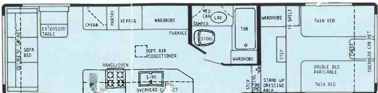
32' Front Bath Doorside Kitchen - Dry Wt. 7500 lbs. - Hitch Wt. 1650 lbs. - Overall Length 32'6"
