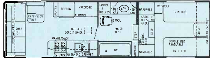
28' Walk-Thru Front Bath - Dry Wt. 6600 lbs. - Hitch Wt. 1650 lbs. - Overall Length 28'8"
