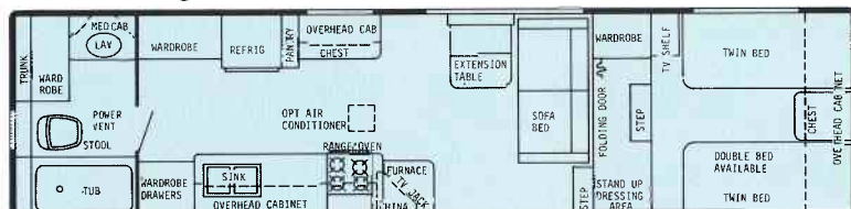
32' Rear Bath Doorside Kitchen - Dry Wt. 7500 lbs. - Hitch Wt. 1650 lbs. - Overall Length 32'6"
