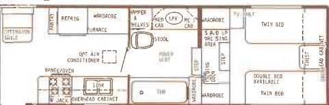
35' Walk-Thru Front Bath - Dry Wt. 6600 lbs. - Hitch Wt. 1450 lbs. - Overall Length 28'8"
