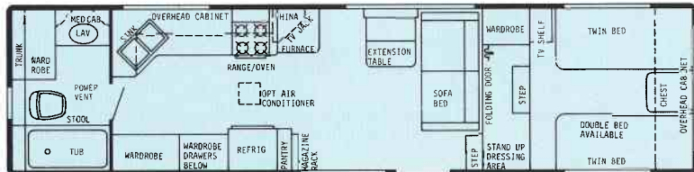
32' Rear Bath - Dry Wt. 7500 lbs. - Hitch Wt. 1650 lbs. - Overall Length 32'6"
