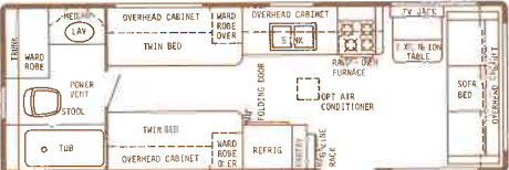
27' Rear Bath - Dry Wt. 5900 lbs. - Hitch Wt. 550 lbs. - Overall Length 27'5"
