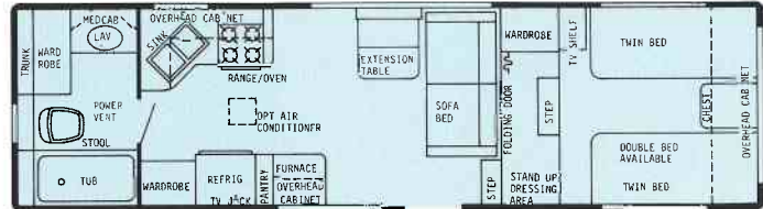
28' Rear Bath - Dry Wt. 6600 lbs. - Hitch Wt. 1650 lbs. - Overall Length 28'8"
