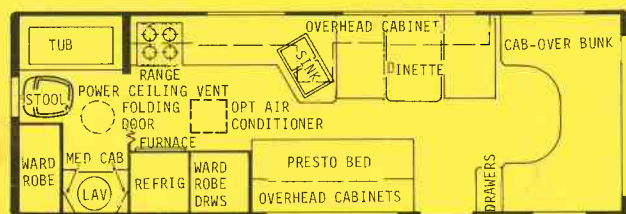
28RB - Dry Wt. 10,000 lbs. - Overall length 27'4"
