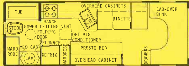
26RB - Dry Wt. 9800 lbs. - Overall length 26'4"
