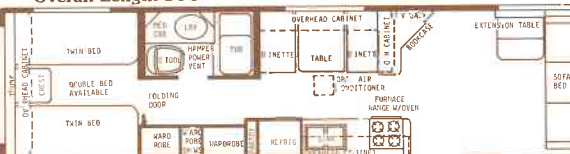
35' Center Bath Dinette - Dry Wt. 7400 lbs. - Hitch Wt. 700 lbs. - Overall Length 34'6"
