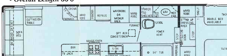
35' Walk-Thru Front Bath - Dry Wt. 8500 lbs. - Hitch Wt. 1650 lbs. - Overall Length 35'6"
