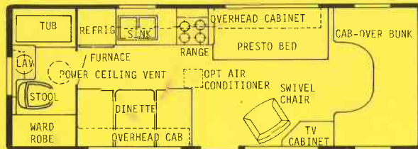
26RBD - Dry Wt. 9800 lbs. - Overall length 26'4"
