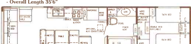
35' Walk-Thru Front Bath 2-Door - Dry Wt. 8500 lbs. - Hitch Wt. 1650 lbs. - Overall Length 35'6"
