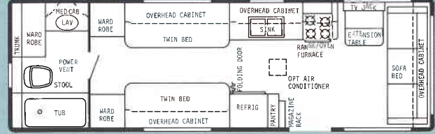
29' Rear Bath - Dry Wt. 6500 lbs. - Hitch Wt. 675 lbs. - Overall Length 29'5"
