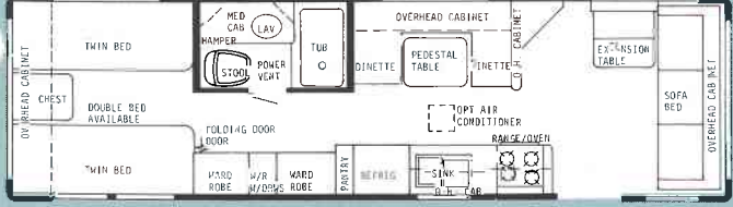
31' Center Bath Dinette - Dry Wt. 6700 lbs. - Hitch Wt. 700 lbs. - Overall Length 31'5"
