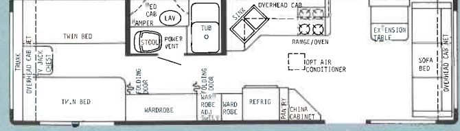
31' Center Bath - Dry Wt. 6700 lbs. - Hitch Wt. 700 lbs. - Overall Length 31'5"
