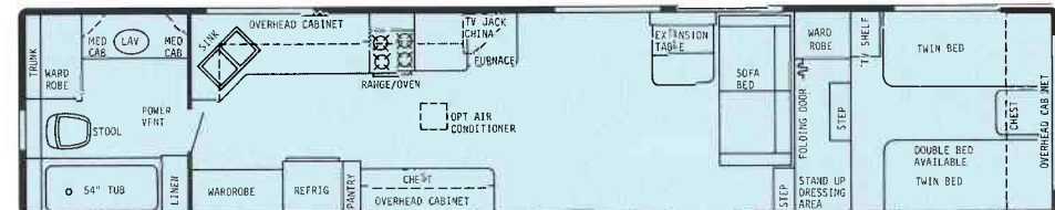
40' Rear Bath Plan #2 - Dry Wt. 9300 lbs. - Hitch Wt. 1750 lbs. - Overall Length 39'6"
