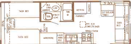
27' Center Bath - Dry Wt. 5900 lbs. - Hitch Wt. 550 lbs. - Overall Length 27'5"
