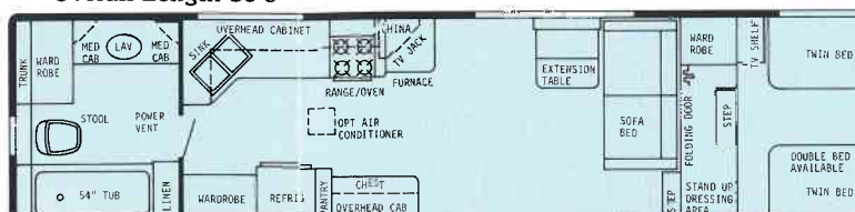
35' Rear Bath Plan #2 - Dry Wt. 8500 lbs. - Hitch Wt. 1650 lbs. - Overall Length 35'6"
