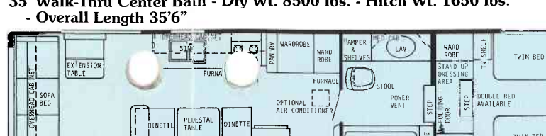
35' Walk-Thru Front Bath 2-Door - Dry Wt. 8500 lbs. - Hitch Wt. 1650 lbs. - Overall Length 35'6"
