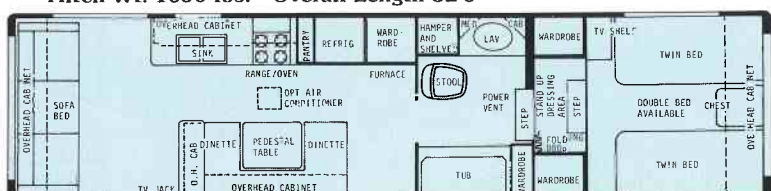
32' Walk-Thru Front Bath 2-Door - Dry Wt. 7500 lbs. - Hitch Wt. 1650 lbs. - Overall Length 32'6"
