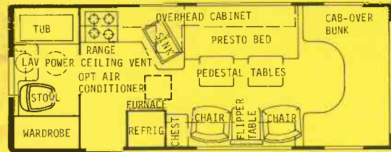
23RBRD - Dry Wt. 9600 lbs. - Overall length 24'4"
