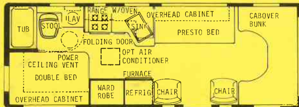
26RBDB - Dry Wt. 9800 lbs. - Overall length 26'4"
