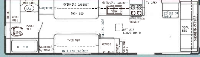
31' Rear Bath - Dry Wt. 6700 lbs. - Hitch Wt. 700 lbs. - Overall Length 31'5"
