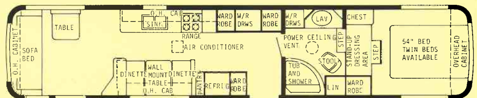
40' Kingsman F.W. - Dry Wt. 8800 lbs. - Hitch Wt. 1750 lbs. - Overall Length 40'
