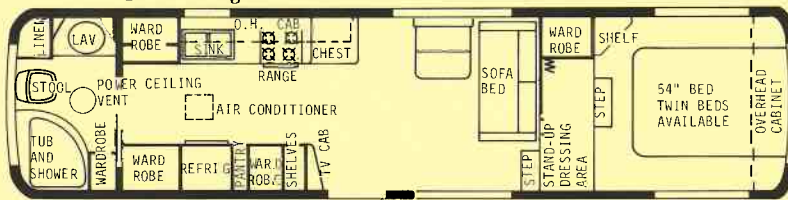
32' Baron F.W. - Dry Wt. 7200 lbs. - Hitch Wt. 1750 lbs. - Overall Length 32' 9"
