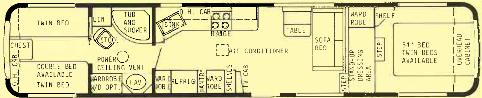
40' Viscount F.W. - Dry Wt. 8800 lbs. - Hitch Wt. 1750 lbs. - Overall Length 40'
