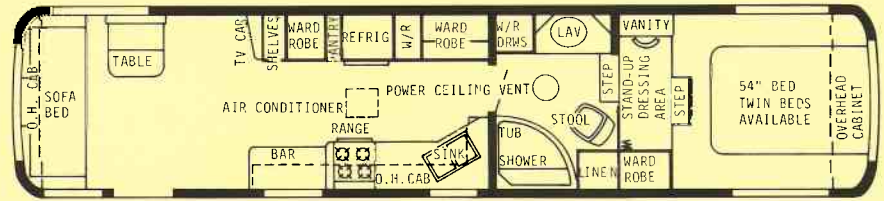
35' Statesman F.W. - Dry Wt. 7600 lbs. - Hitch Wt. 1800 lbs. - Overall Length 35' 9"
