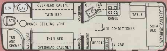
29' Baron T.T. - Dry Wt. 5700 lbs. - Hitch Wt. 800 lbs. - Overall Length 29' 8"
