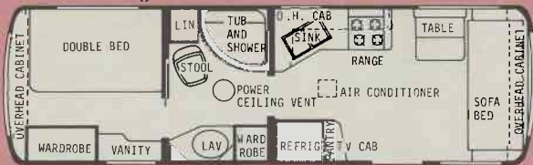
29' Viscount T.T. - Dry Wt. 5700 lbs. - Hitch Wt. 800 lbs. - Overall Length 29' 8"
