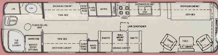
35' Baron TT - with Dinette
