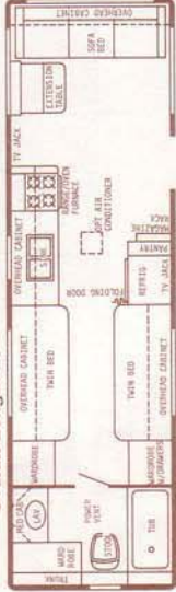
29' Center Bath - Dry Wt. 6500 lbs. - Hitch Wt. 675 lbs. - Overall Length 29'5"
