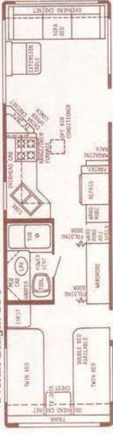
33' Center Bath Dinette - Dry Wt. 6900 lbs. - Hitch Wt. 700 lbs. - Overall Length 33'5"
