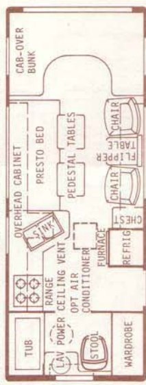
23RB - Dry Wt. 9600 lbs. - Overall length 24'4"
