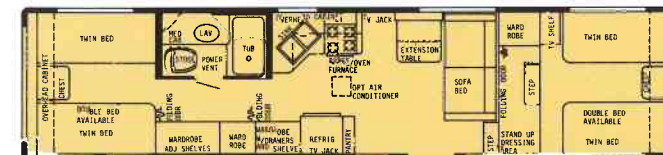
35' Center Bath - Dry Wt. 8500 lbs. - Hitch Wt. 1650 lbs. - Overall Length 35'6"
