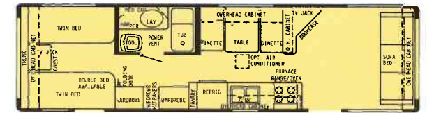
33' Center Bath Dinette - Dry Wt. 6900 lbs. - Hitch Wt. 700 lbs. - Overall Length 33'5"
