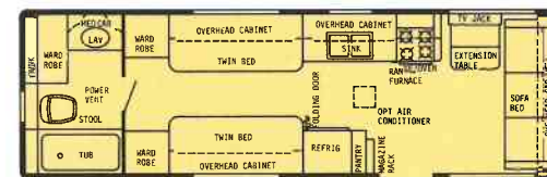
29' Rear Bath - Dry Wt. 6500 lbs. - Hitch Wt. 675 lbs. - Overall Length 29'5"
