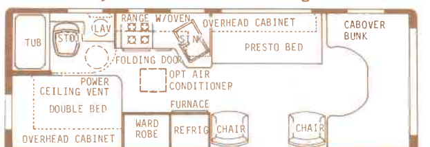
26RBDB - Dry Wt. 9800 lbs. - Overall length 26'4"
