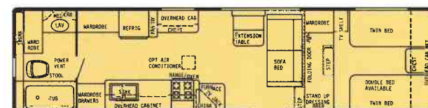
32' Rear Bath Doorside Kitchen - Dry Wt. 7500 lbs. - Hitch Wt. 1750 lbs. - Overall Length 32'6"
