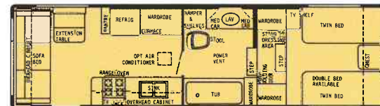
28' Walk-Thru Front Bath - Dry Wt. 6600 lbs. - Hitch Wt. 1450 lbs. - Overall Length 28'8"
