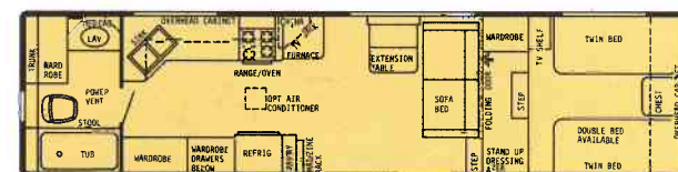
32' Rear Bath - Dry Wt. 7500 lbs. - Hitch Wt. 1750 lbs. - Overall Length 32'6"
