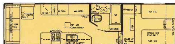
32' Front Bath Doorside Kitchen - Dry Wt. 7500 lbs. - Hitch Wt. 1750 lbs. - Overall Length 32'6"
