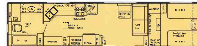
35' Rear Bath Plan #1 - Dry Wt. 8500 lbs. - Hitch Wt. 1750 lbs. - Overall Length 35'6"
