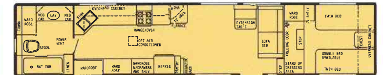
40' Rear Bath Plan #1 - Dry Wt. 9300 lbs. - Hitch Wt. 1650 lbs. - Overall Length 39'6"
