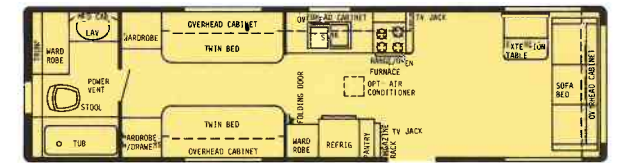
33' Rear Bath - Dry Wt. 6900 lbs. - Hitch Wt. 700 lbs. - Overall Length 33'5"
