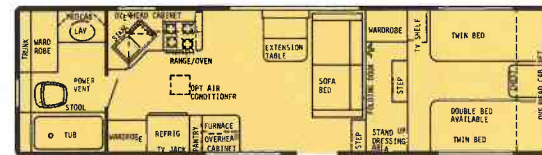
28' Rear Bath - Dry Wt. 6600 lbs. - Hitch Wt. 1650 lbs. - Overall Length 28'8"
