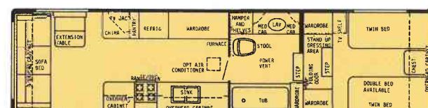
32' Walk-Thru Front Bath - Dry Wt. 7500 lbs. - Hitch Wt. 1750 lbs. - Overall Length 32'6"
