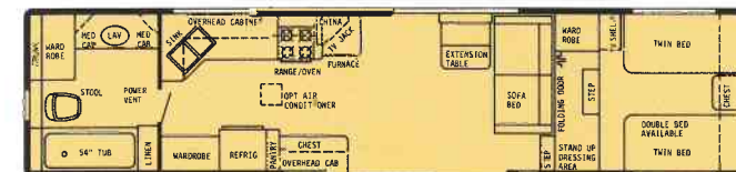
35' Rear Bath Plan #2 - Dry Wt. 8500 lbs. - Hitch Wt. 1750 lbs. - Overall Length 35'6"
