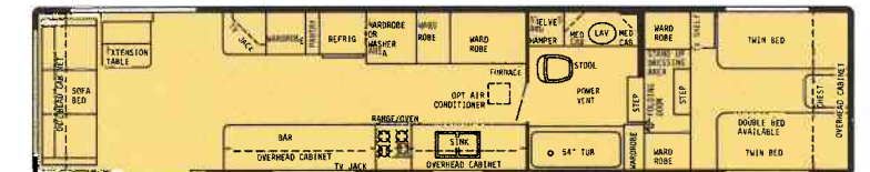
40' Walk-Thru Front Bath - Dry Wt. 9300 lbs. - Hitch Wt. 1650 lbs. - Overall Length 39'6"
