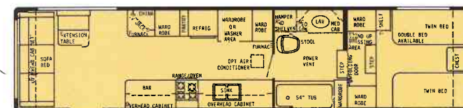
35' Walk-Thru Front Bath - Dry Wt. 8500 lbs. - Hitch Wt. 1650 lbs. - Overall Length 35'6"
