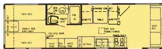
31' Center Bath Dinette - Dry Wt. 6700 lbs. - Hitch Wt. 700 lbs. - Overall Length 31'5"
