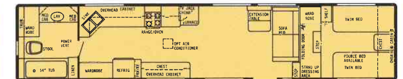
40' Rear Bath Plan #2 - Dry Wt. 9300 lbs. - Hitch Wt. 1650 lbs. - Overall Length 39'6"
