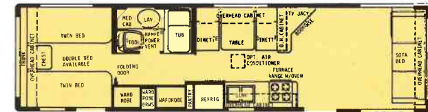
35' Center Bath Dinette - Dry Wt. 7400 lbs. - Hitch Wt. 700 lbs. - Overall Length 34'6"
