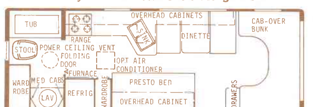
26RB - Dry Wt. 9800 lbs. - Overall length 26'4"
