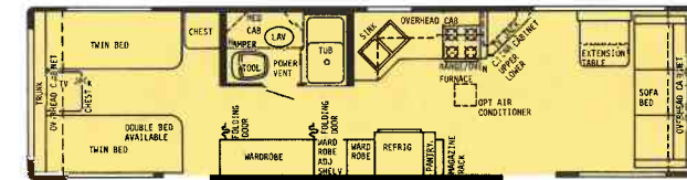
35' Center Bath - Dry Wt. 7400 lbs. - Hitch Wt. 700 lbs. - Overall Length 34'6"
