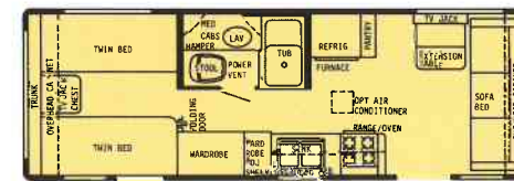
27' Center Bath - Dry Wt. 5900 lbs. - Hitch Wt. 550 lbs. - Overall Length 27'5"
