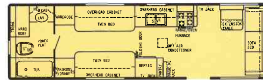
31' Rear Bath - Dry Wt. 6700 lbs. - Hitch Wt. 700 lbs. - Overall Length 31'5"
