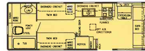
27' Rear Bath - Dry Wt. 5900 lbs. - Hitch Wt. 550 lbs. - Overall Length 27'5"
