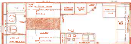
27' Rear Bath Travel Trailer Dry Weight - 4400 lbs. Hitch Weight - 500 lbs. Overall Length - 26' 11"
